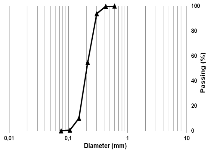
Figure 5 Grading curve of Fontainebleau sand.
