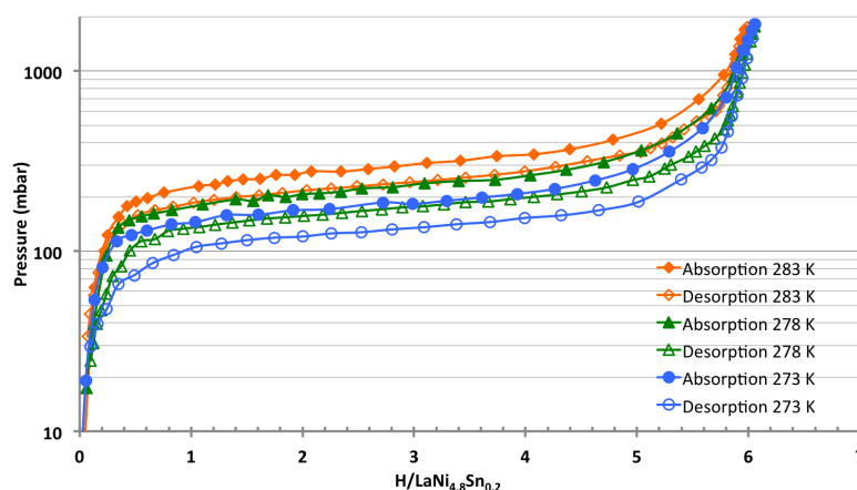
Figure 3. PCT curves for the LaNi_{4.8}Sn_{0.2} powder synthesized at CNRS/Inst. Néel and used for hydrogen gas storage.
