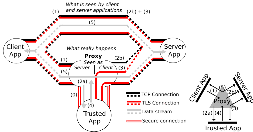
Figure 4: Establishment of TLS Switching connections.
