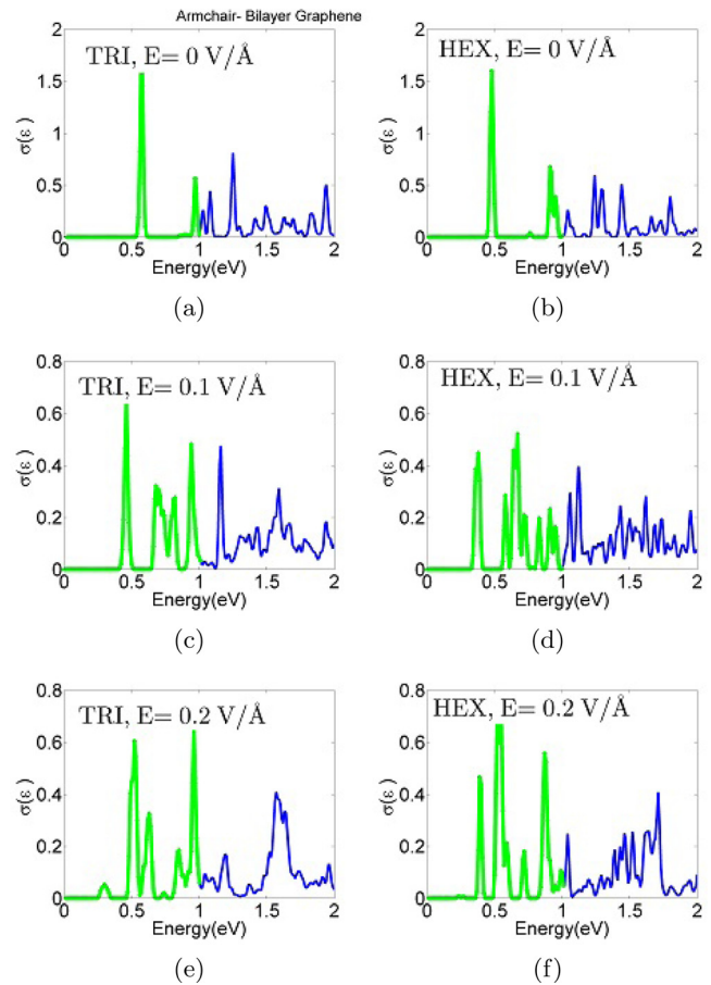
FIG. 10. Optical absorption spectra for armchair bilayer graphene QDs of triangular (a), (c), (e) and hexagonal (b), (d), (f) shapes with 720 ( L \approx 64 \text{ \AA} ) and 762 ( L \approx 27 \text{ \AA} ) atoms per layer, respectively.
