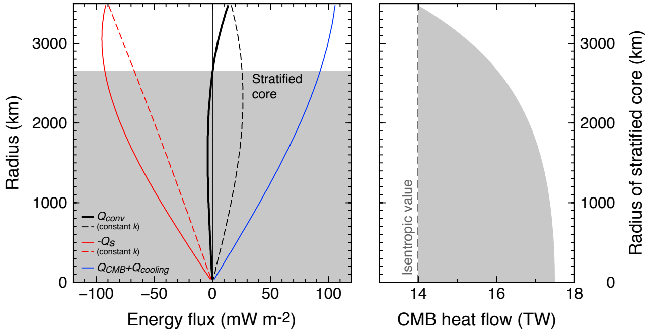
Figure 10: Radial profiles of contributions to the convective heat flux density (A) and limit to the region with negative convective heat flow as function of the CMB value (B) for the period just preceding the onset of inner core crystallization. The profiles are computed for Q_{CMB} = 16.1\text{TW} for an isentropic value Q_S = 14\text{TW} . The dashed lines are obtained for constant value of the thermal conductivity, equal to the CMB value, and show no stratification.
