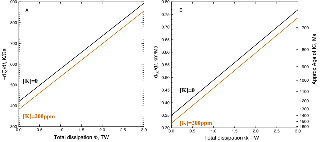
Figure 3: Core cooling rate just before the onset of inner core crystallization (A) and present inner core growth rate (B) as function of total dissipation. Also given on the right axis of B is the approximate age of the inner core, in Myr. See § 3.4 for details of this calculation.
