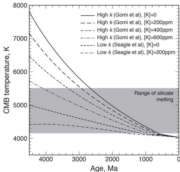
Figure 13: Evolution of the CMB temperature with time for the model presented on figure 11 (solid line) as well as cases with varying amounts of potassium in the core and for the conductivity value proposed by Seagle et al. (2013), as labeled. The shaded area corresponds to the approximate range between the solidus and the liquidus for a “chondritic mantle” (Andraut et al., 2011) or a peridotite (Fiquet et al., 2010).
