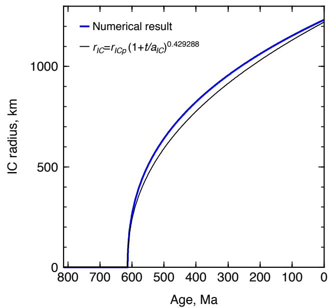
Figure 5: Typical example of inner core growth curve showing that it follows a power law with an exponent close to 0.4.
