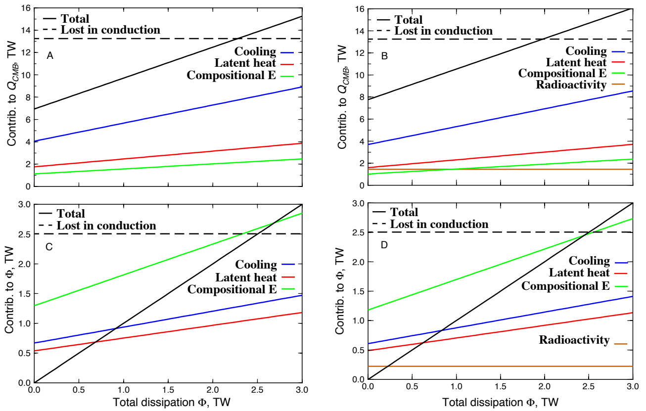
Figure 6: Contributions to the core energy balance (A and B) and dissipation (C and D) as a function of the wanted total dissipation for the present period, with inner core crystallization, without any radioactivity (A and C) or including 200 ppm of potassium (B and D).
