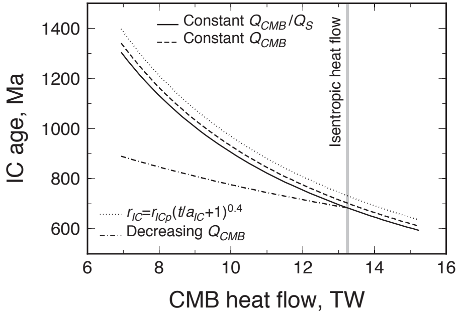
Figure 7: Age of the inner core as function of the present CMB heat flow. The solid line is obtained assuming a linear evolution of the CMB heat flow keeping the same ratio to the isentropic value while the dashed line assumes a constant CMB heat flow. The dotted line is obtained from just the present inner core growth rate and assuming a power law growth history. The dash-dotted line is obtained assuming a linearly decreasing CMB heat flow between the isentropic value at the onset of the inner core and the present value given in abscissa. The vertical grey line gives the present time value of the isentropic heat flow at the CMB. See text for details.
