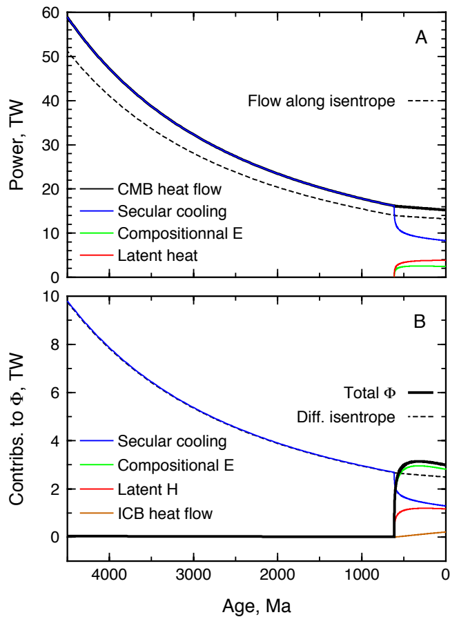
Figure 11: Evolution of the contributions to the the CMB heat flow (A) and total dissipation (B) as function of time for a CMB heat flow that is always 1.15 times the isentropic value.
