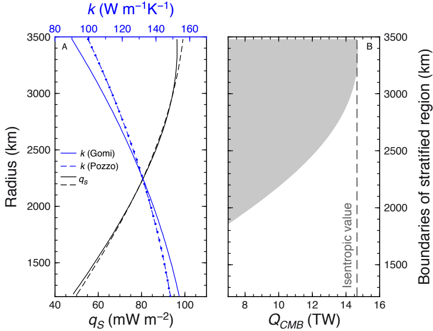
Figure 9: (A) Comparison of profiles of thermal conductivity and isentropic heat flux between the present work and that of Pozzo et al. (2012) and Gubbins et al. (2015). The solid blue line is the same conductivity as that presented on figure 2, for reference, the blue dots are the conductivity values from Pozzo et al. (2012) and the dashed blue line is the fit of these values according to equation (20). The dashed black line is the isentropic heat flux density of Pozzo et al. (2012) while the solid black line is obtained with the temperature profile used in the present study and the conductivity of Pozzo et al. (2012). (B) Radial boundaries of the predicted stratified layer as a function of the CMB heat flow obtained using the conductivity profile of Pozzo et al. (2012).
