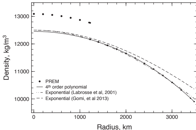
Figure 1: Density as function of radius in the core. Circles are the PREM values, the solid line is the 4 th order fit according to equation (5) with parameters given in table 2. The dashed line and dash-dotted line are exponential forms \rho = \rho_0 \exp(-r^2/L^2) using L = 7765\text{km} and L = 7400\text{km} , respectively.
