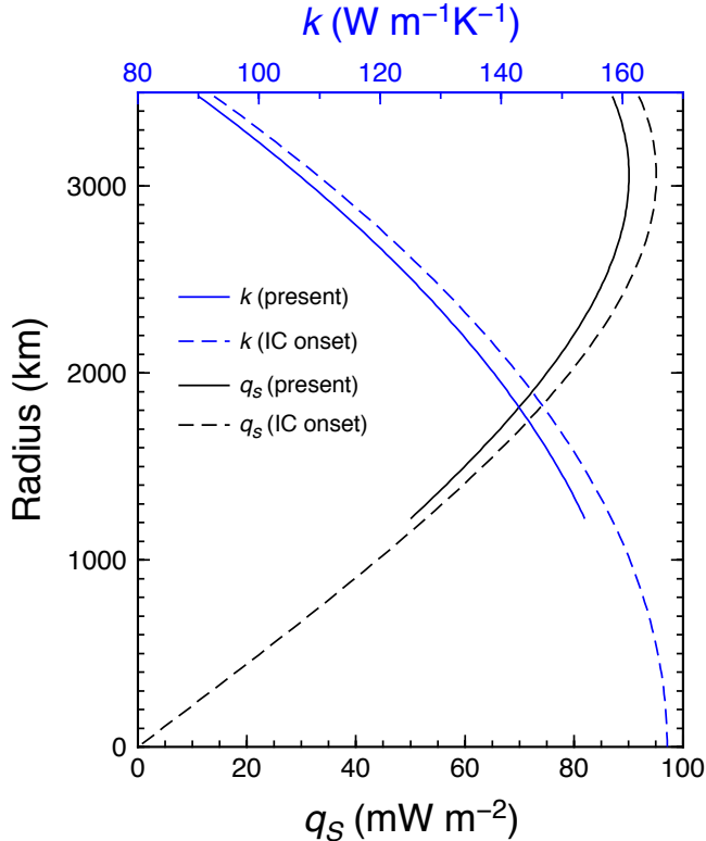
Figure 2: Profiles of thermal conductivity ( k , blue, top scale) and isentropic heat flux density ( q_s \equiv -k\partial_r T_a black, bottom scale) as function of radial position in the core. Solid lines are for the present time while dashed lines are for the onset time of the inner core.
