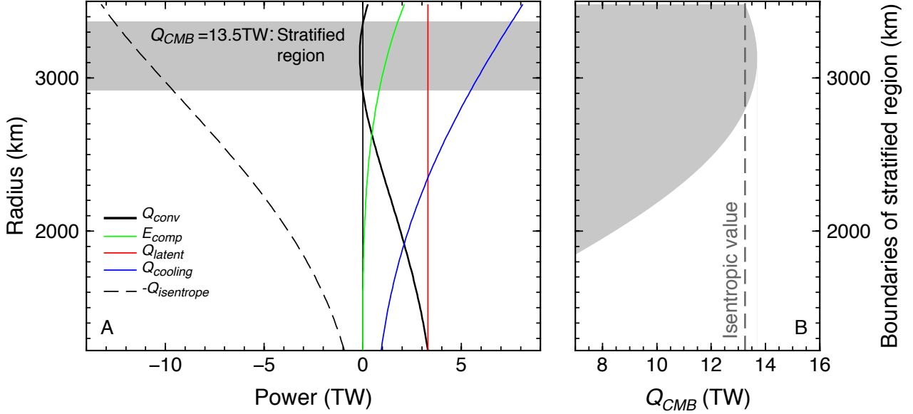
Figure 8: Radial profiles of contributions to the convective heat flow (A) and limits to the region with negative convective heat flow as function of the present time CMB heat flow value (B). The profiles are computed for Q_{CMB} = 13.5\text{TW} , that is slightly larger than the isentropic value ( Q_S = 13.25\text{TW} ).
