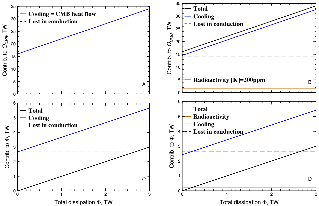
Figure 4: Contributions to the core energy balance (A and B) and total dissipation (C and D) as a function of the wanted total dissipation for the period just preceding the onset of the inner core crystallization, without any radioactivity (A and C) or including 200 ppm of potassium (B and D).
