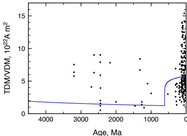
Figure 12: Evolution of the predicted dipole moment for the thermal evolution presented on figure 11 (solid blue line) and of the measured virtual dipole moments (dots, same selection as by Aubert et al., 2009). Note that the expected increase of the dipole field is small compared to the observed fluctuations and would be hardly detectable. See text for a discussion.
