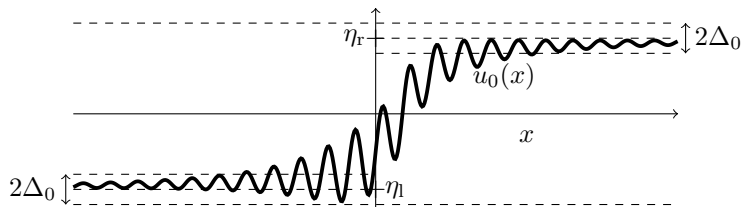
Figure 3: A possible initial condition u_0 in Theorem 1.3.
