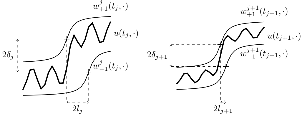
Figure 4: Squeezing of u(t, x) solution to (5).
