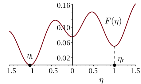
Figure 2: A double-well “camel-hump” potential F , \eta_l = -1 , \eta_r = 1 .
