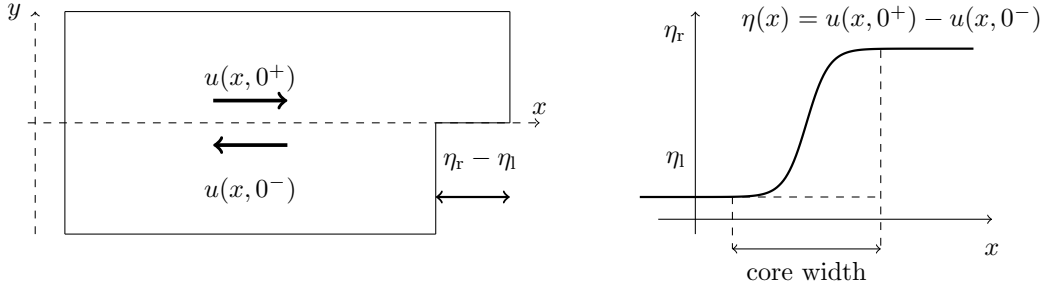
Figure 1: Typical shape of \eta(x) , solution to (1); here, u(x, y) is the material displacement.
