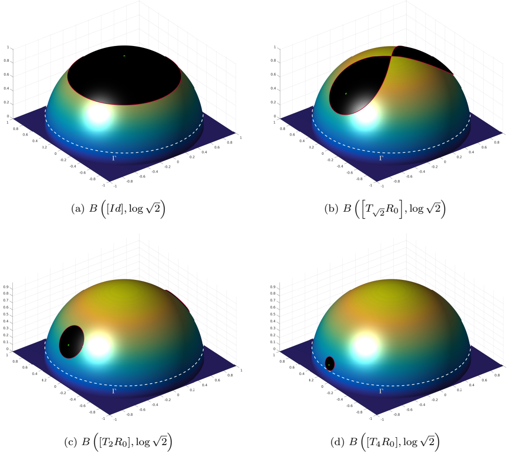
Figure 4: (Perspective views) Green point - Affine transformation in question Dashed line - \partial B\left([Id], \log 4\sqrt{2}\right) Black surface - Disk in question
