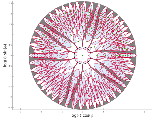
(f) Proposed covering in [35], called HARD Configuration for SURF-SURF. This is a log 1.5-covering of \{[T_t R_\phi] \mid t \leq 1.5\} with 112 affine simulations representing an area ratio of 21.28.
