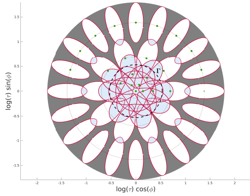
(b) Proposed covering for FAIR-SURF in [44], called fixed tilts. This is a log 1.5-covering of \{[T_t R_\phi] \mid t \leq 1.7\} with 23 affine simulations representing an area ratio of 11.42.
