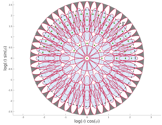
(e) Proposed covering in [35], called HARD configuration for DoG-SIFT. This is a log 1.8-covering of \{[T_t R_\phi] \mid t \leq 9.6\} with 61 affine simulations representing an area ratio of 13.
