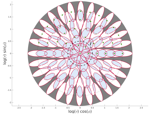
(c) Proposed covering for FAIR-SURF in [44], called simulated tilts. This is a log 1.5-covering of \{[T_t R_\phi] \mid t \leq 1.65\} with 41 affine simulations representing an area ratio of 13.77.
