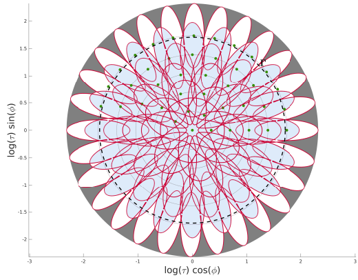
(a) Proposed covering for ASIFT in [39, 59]. This is a log 1.8-covering of \{[T_t R_\phi] \mid t \leq 5.5\} with 41 affine simulations representing an area ratio of 13.77.
