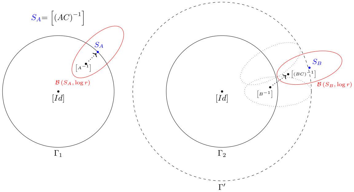
Figure 5: Sketch of the proof of Theorem 18.
