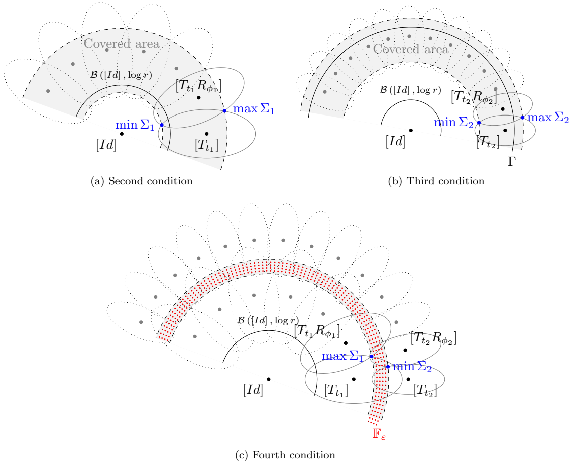
Figure 8: Verifying covering conditions for feasible sets in Proposition 30.
