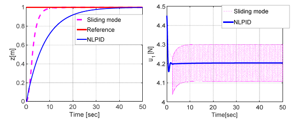
Figure 3: Comparison in vertical flight.
