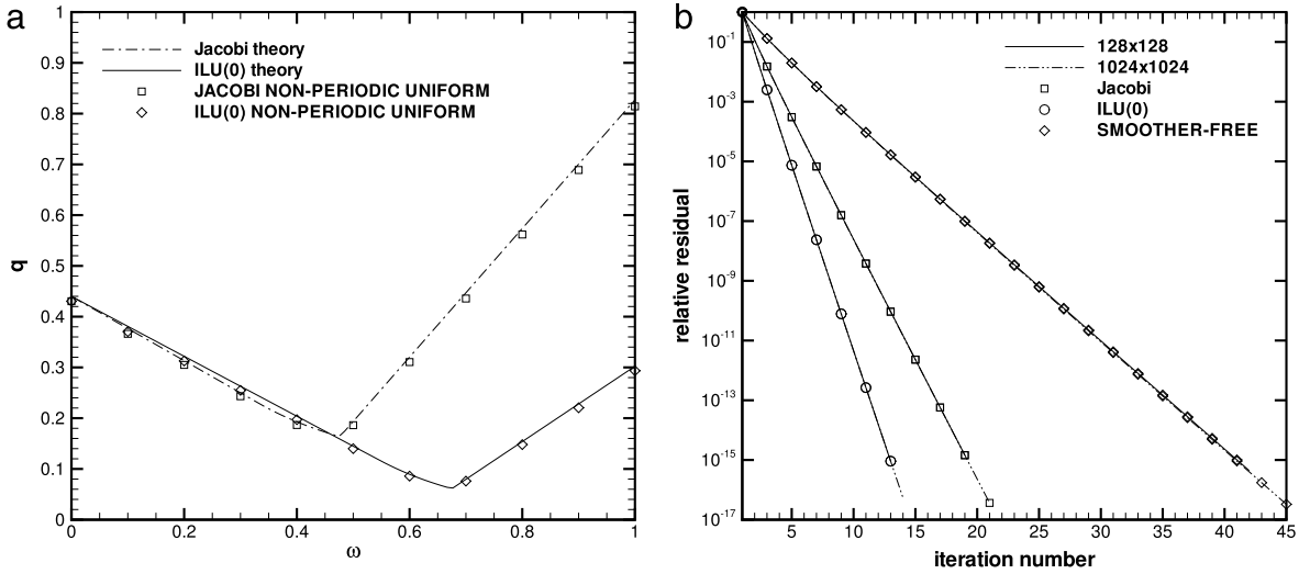
Fig. 5. Convergence factor versus relaxation factor (a), defect reduction versus the iteration number (b) with Neumann boundary conditions and uniform meshes.
