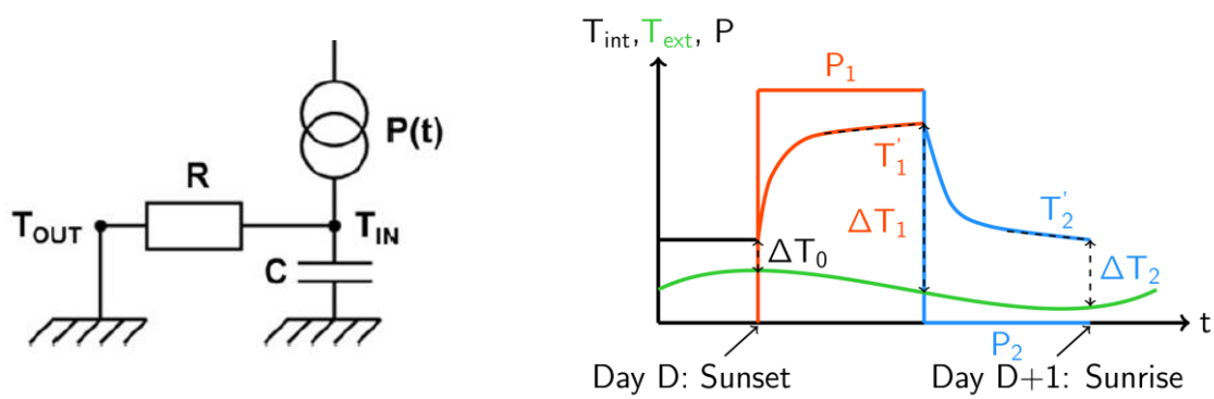
Figure 1: RC model used in the QUB method (left) and evolution of temperature and power during a QUB measurement (right)
