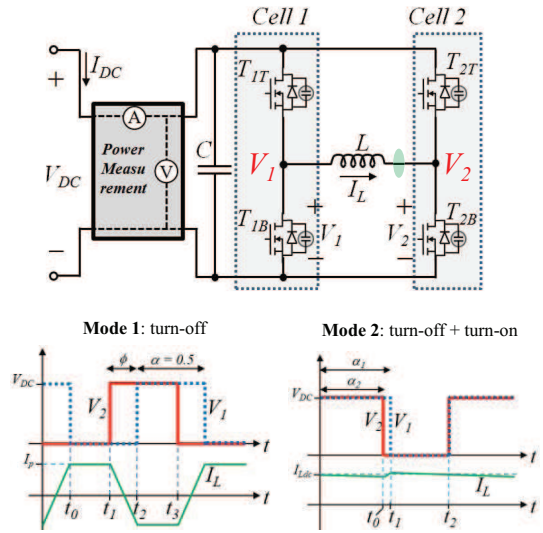
Fig. 2. Operating principle of the characterisation method.
