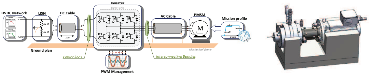
Fig. 1. Electromechanical Drive in the normative conditions according to the DO-160 Standard & Coupled electrical motors.
