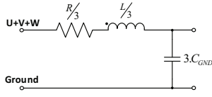
Fig. 10. CM equivalent circuit of the AC Cable.
