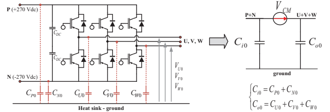
Fig. 9. Equivalent circuit of the inverter (CM point of view).
