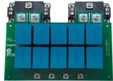
Fig. 3. Developed test board used for switching energy measurement specifically designed for the CAS100H12AM1 modules.
