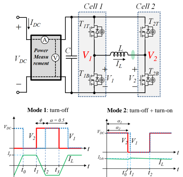
Fig. 2. Operating principle of the characterisation method.
