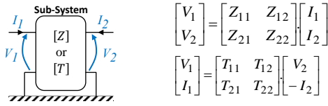
Fig. 15. Two port networks representation.
