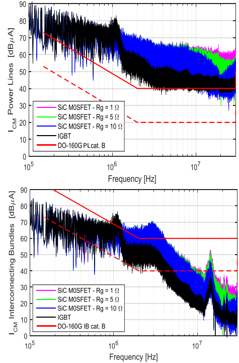
Fig. 17. CM currents at inverter input and output ( F_{sw} = 15 kHz, I_{out} = 20 A).
