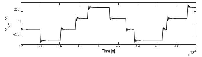
Fig. 8. Analytical CM Voltage waveform.
