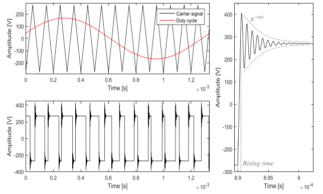
Fig. 7. Mathematical generation of output phase voltage waveform.
