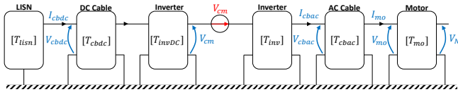
Fig. 16. Common mode quadripolar chain.
