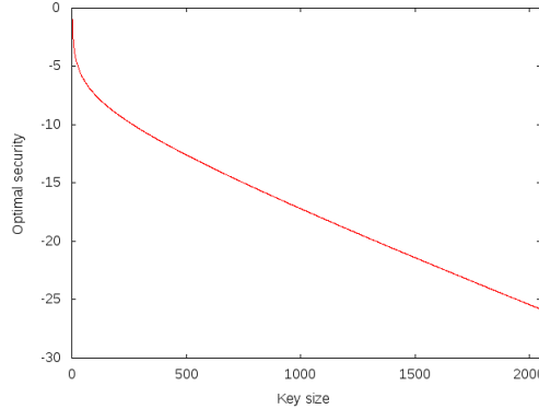
Fig. 5 The base-2 log of a lower bound for the best attack probability on HB+DB for \mathbb{P}_{FR} = 0.01 and k sessions, for each key size k .
