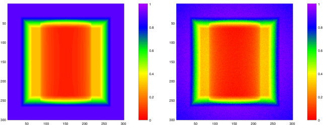
(a) Deterministic simulated image using gVirtualXRay. (b) MC simulated image using Geant4.
