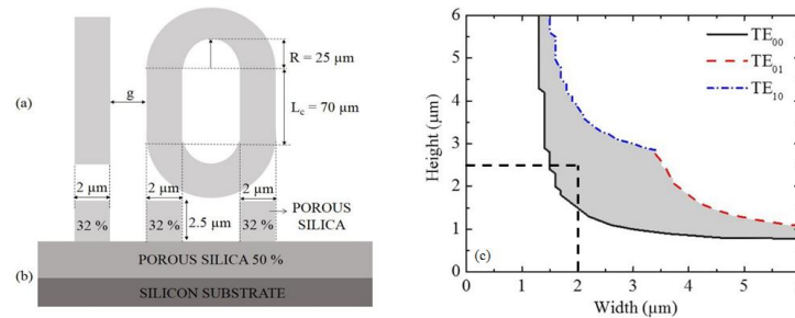
Figure 1: Schema of a top view (a) and a cross section (b) of the porous silica racetrack MR. (c) Solutions of the Maxwell equations for the TE_{00} , TE_{01} and TE_{10} modes as a function of the porous silica ridge waveguide dimensions.
