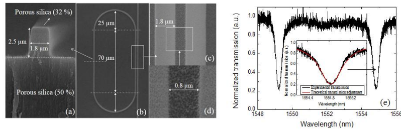
Figure 2: SEM images of the racetrack resonator: (a) cross section of a porous silica ridge waveguide; top views at different scales of : (b) the whole racetrack MR, (c) the two waveguides in the coupling area and (d) the gap separation between the two waveguides of the coupling area. (e) Experimental transmission spectra for one polarization of light. In the insert, the theoretical transmission is adjusted to the experimental one.
