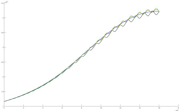
Fig. 5. Dynamics with full perturbations, case of a rendez-vous in (a, e, \omega, \Omega, i) . Plot of the semi-latus rectum P for \Delta = 2\pi (blue curve), \Delta = \pi (red curve), \Delta = \pi/2 (green), and for the true dynamics (black curve).
