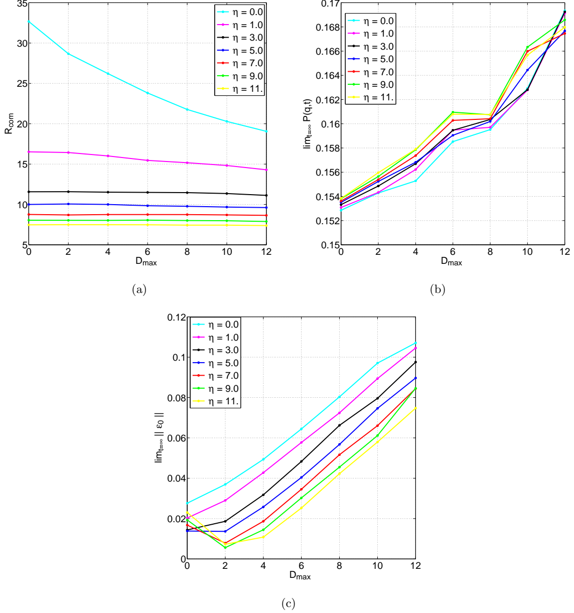
Fig. 6. Evolution of R_{\text{com}} , P(q,t) and \varepsilon_0 for different values of D_{\text{max}} \in \{0, 2, 4, 6, 8, 10, 12\} , \eta \in \{0, 1, 3, 5, 7, 9, 11\} and \eta_2 = 7.5 . Model (41) and constant estimator (42)-(43) are considerate.
