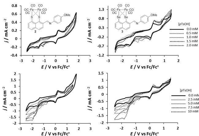
Figure 4. Cyclic voltammograms for [FeFe] complexes 2 and 3 (1 mM) in 0.1 M \text{NBu}_4\text{PF}_6/\text{CH}_3\text{CN} at 0.01 \text{ V s}^{-1} scan rate with increasing concentrations of p\text{TsOH} from 0.5 mM to 2 mM (upper graphs) and from 2.5 mM to 10 mM (lower graphs).
