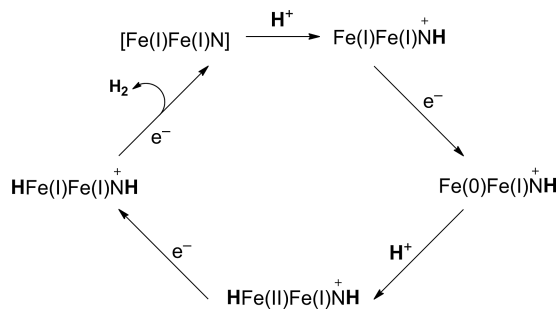
Scheme 3. Proposed mechanism for the proton reduction catalysis by [FeFe] complexes 2 and 3 in the presence of p\text{TsOH} .
