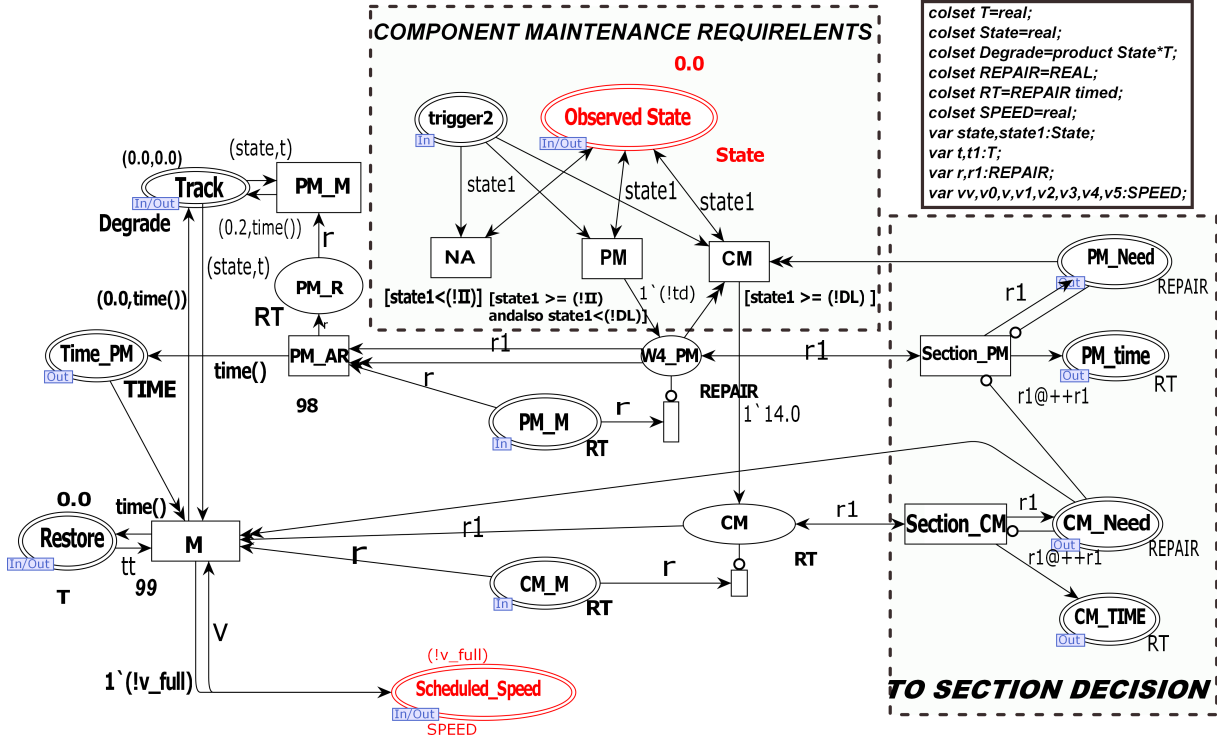
Figure 9: Track deterioration CPN model
