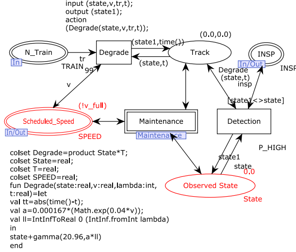
Figure 9: Track deterioration CPN model
