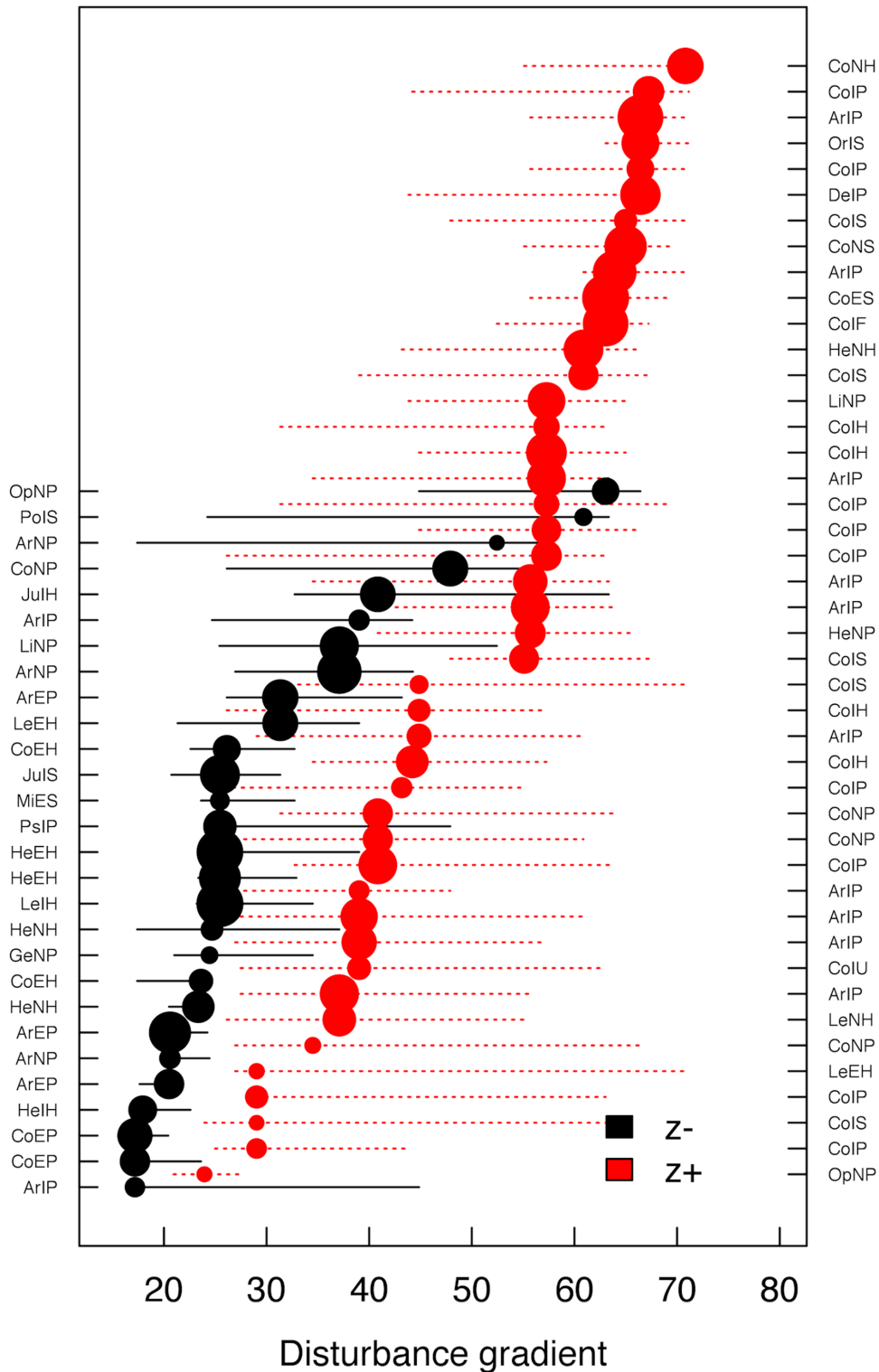
Figure 2. Change points and 90% confidence limits of significant indicator species (n=72) along the disturbance gradient. Significant indicator species are species with, \text{IndVal } p < 0.05 , purity > 0.95 and reliability > 0.95 for 500 bootstrap and 250 permutation replicates. Change points are represented by black and red circles for species associated with low and high disturbance respectively and are sized in proportion to the magnitude of the response (z scores; see Materials and methods). Code for species on vertical axis (both left and right): The two first letters: Order (e.g. Ar = Araneae, He = Hemiptera, etc.; see Supporting Information S1); the third letter is the biogeographic category (E = endemic, N = Native non-endemic and I = Introduced/Exotic). The last letter is the feeding guild (P = predator, H = herbivore, F = Fungivore, S = Saprophagous and U = Undetermined).
