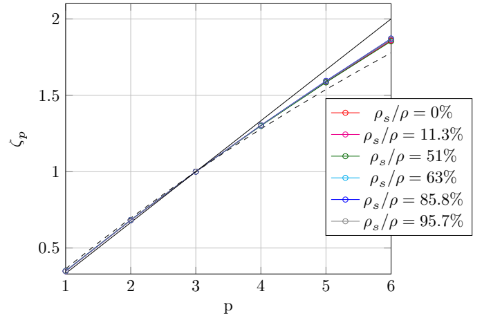
FIG. 9. Experimental exponent computed using the ESS method (coloured circles). The error bars corresponding to the fit uncertainty reported in Table III are not plotted because there are smaller than the size of the circle symbols. For comparison, are also plotted exponents \zeta_p = p/3 expected with no intermittency (black line), and those from the She-Lévêque model [39] ( \zeta'_p = \frac{p}{9} + 2[1 - (\frac{2}{3})^{p/3}] ), predicted using the standard definition of exponents (dashed curve).
