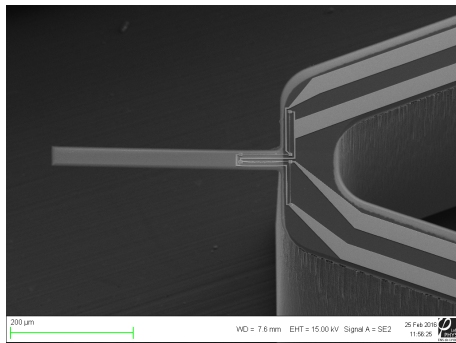
(b) Electronic microscope image of the cantilever
