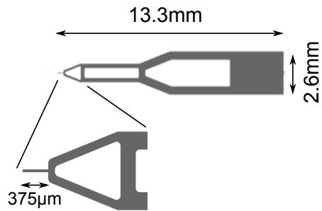
(a) Sketch of a cantilever probe
