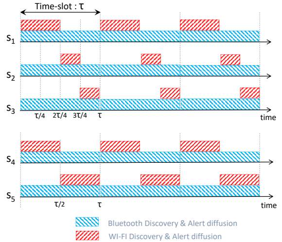
Fig. 2. Wake-up schedule
