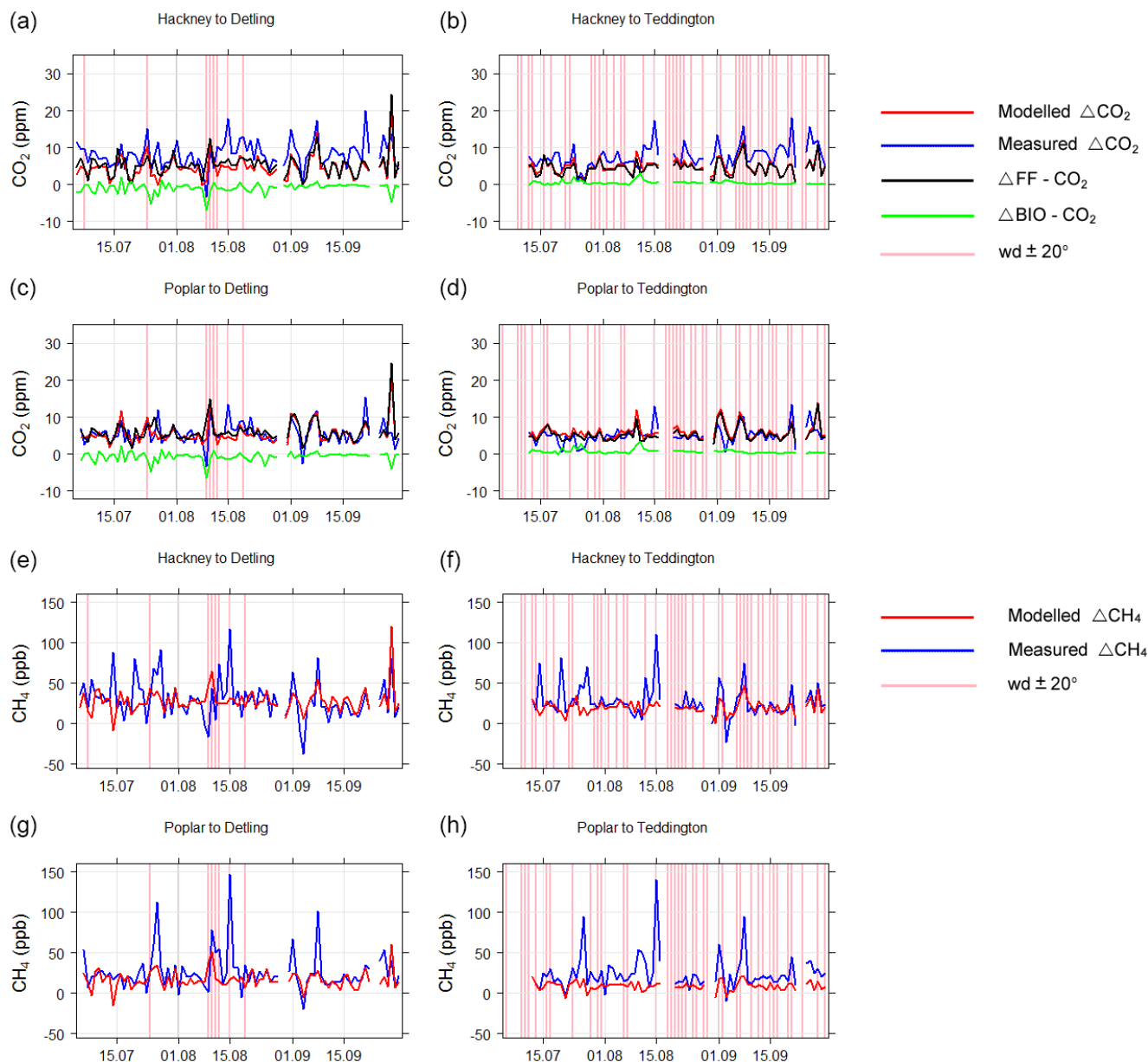
Figure 6. Time series of averages for the afternoon period (12:00 to 17:00 UTC) each day of measured \Delta\text{CO}_2 (blue), modelled \Delta\text{CO}_2 (red), modelled signature of the fossil fuel \text{CO}_2 emissions ( \Delta\text{FF-CO}_2 ) (black) and modelled signature of the \text{CO}_2 NEE ( \Delta\text{BIO-CO}_2 ) (green) between (a) Hackney and Detling, (b) Hackney and Teddington, (c) Poplar and Detling and (d) Poplar and Teddington. Time series of averages for the afternoon period (12:00 to 17:00 UTC) of measured (blue) or modelled (red) \Delta\text{CH}_4 between (e) Hackney and Detling, (f) Hackney and Teddington, (g) Poplar and Detling, and (h) Poplar and Teddington. Vertical pink lines indicate days during which at least one hourly afternoon wind direction is within a \pm 20^\circ range around the direct line from the reference site to the urban site according to the wind measurements at Heathrow (if the reference site is Teddington) or East Malling (if the reference site is Detling).
