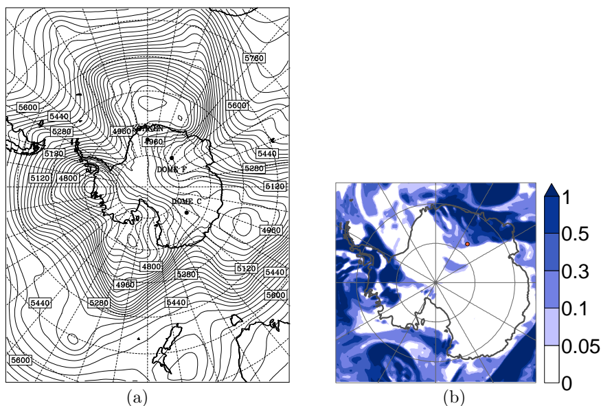
Figure 5. Example of an amplified high-pressure ridge: (a) 500 hPa geopotential height from AMPS, 1 August 2003 12:00 UTC, (b) 6 h precipitation in mm from AMPS, 1 August 2003 06:00 UTC.
