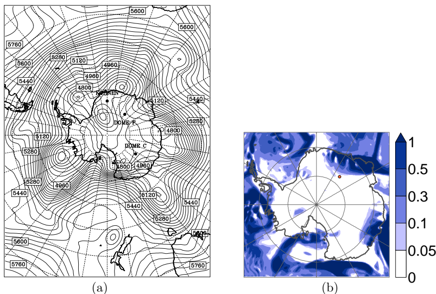
Figure 6. Example of a weak high-pressure ridge: (a) 500 hPa geopotential height from AMPS, 13 August 2003 12:00 UTC, (b) 6 h precipitation in mm from AMPS, 14 August 2003 00:00 UTC.
