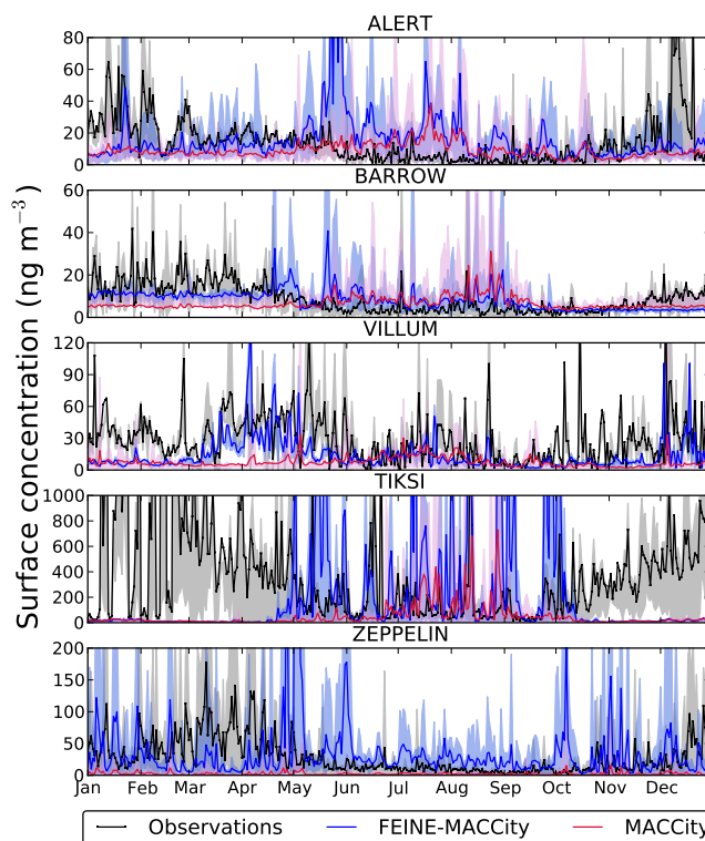
Figure 7. Modelled vs. measured surface concentrations of BC ( \text{ng m}^{-3} ) for the FEI-NE+MACCcity and MACCcity simulations in the Arctic stations Alert, Barrow, Villum, Tiksi, and Zeppelin. Due to the high variability of the surface concentrations, the results are presented as minimum, average, maximum modelled (FEI-NE+MACCcity and MACCcity) and measured surface daily concentrations of BC for the period 2002–2013.
