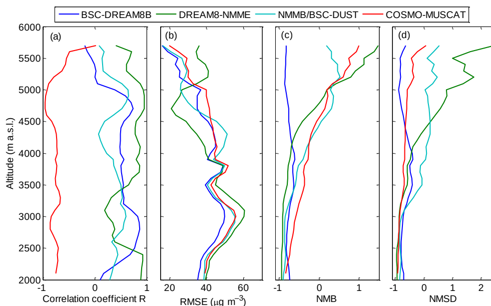
Figure 13. Vertical profiles of the correlation coefficient between LIRIC and the model time series for every altitude level, the root mean square error RMSE, the normalized mean bias NMB, and the normalized mean standard deviation NMSD.
