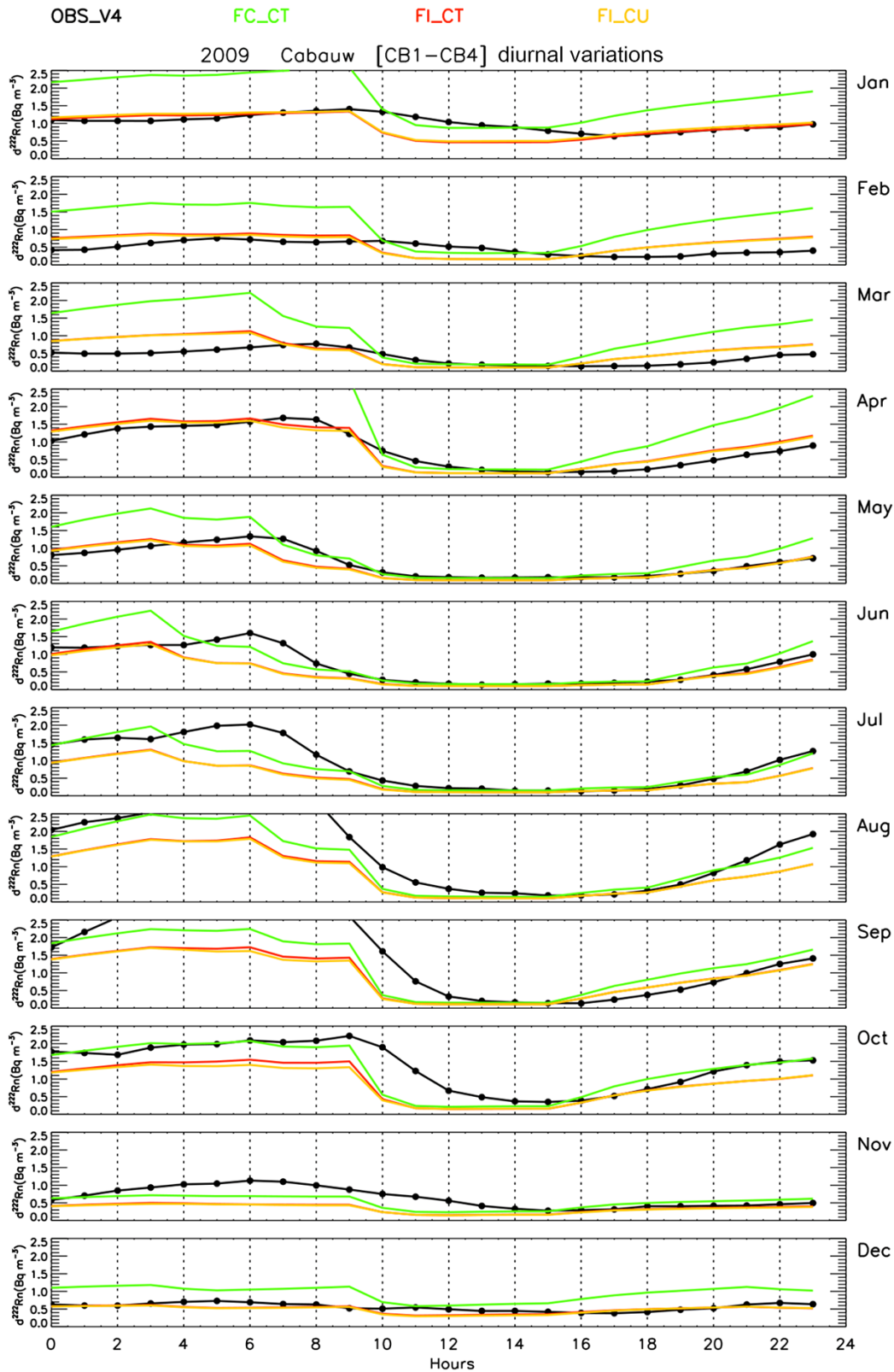
Figure 11. Mean diurnal variations of the radon activity concentration differences between the two measurement levels at Cabauw (20 m (CB1), 200 m (CB4)). The observed gradient is shown by the black solid line with dots (for each month of the year 2009), and the modelled gradient by the solid green line for the constant emissions (FC_CT), by the solid red line for the InGOS emissions (FI_CT), and by the solid orange line for the simulations using the InGOS emissions and the combination of the “revised slopes scheme” and the new convection scheme based on ECMWF reanalyses (FI_CU), respectively.
