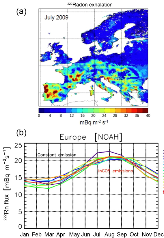
Figure 2. Radon ( ^{222}\text{Rn} ) emissions used for the model simulations, (a) spatial distribution of InGOS emissions over Europe during July 2009, (b) seasonal and inter-annual variations of InGOS emissions (in different colours for different years; mean in red) and the commonly used constant emissions (black). The mean seasonal variations are averaged over the geographic domain between 10^\circ W and 30^\circ E longitude and between 35 and 70^\circ N latitude.
