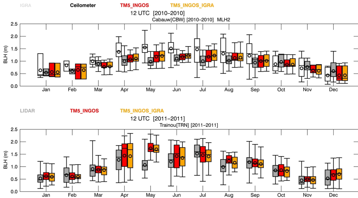
Figure 5. As in Fig. 3, but on the top Cabauw (CBW) where both ceilometer and nearby IGRA observations (from De Bilt) are available. Observed (IGRA in blank; ceilometer in grey) and simulated (colours) boundary layer heights at 12:00 UTC and for 2010 are shown. On the bottom, Trainou (TRN) lidar-based boundary layer heights (grey) at 12:00 UTC during 2011 are shown. The model boundary layer heights are represented by the coloured boxes (for the different acronyms see Sect. 3.2).
