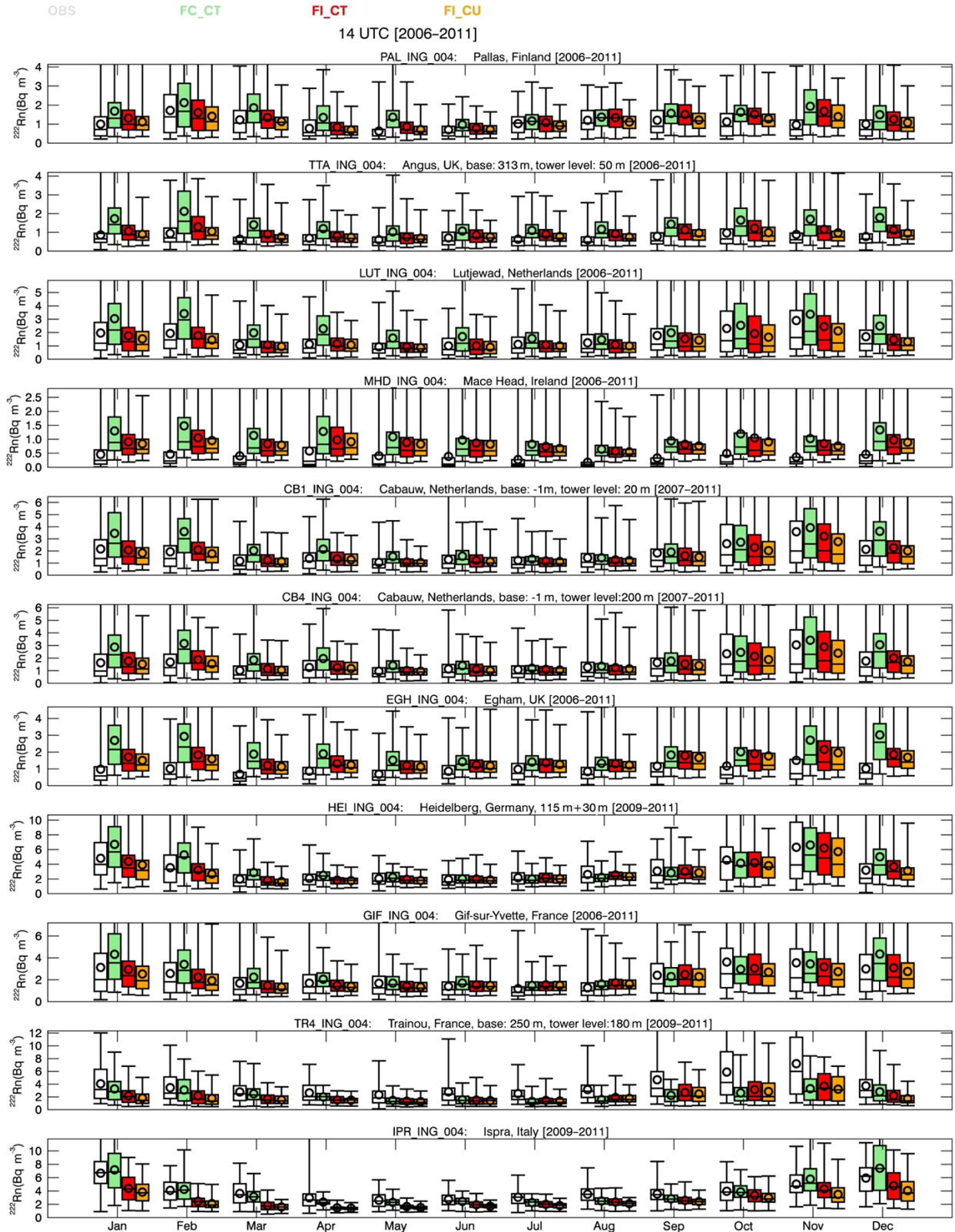
Figure 7. As in Fig. 6, but at 14:00 UTC illustrating the seasonal variations of daily minimum of radon ( ^{222}\text{Rn} ) activity concentrations.
