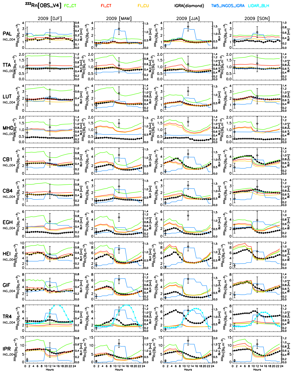
Figure 9. Seasonal variations of ^{222}\text{Rn} activity concentrations and boundary layer heights (BLHs) at the InGOS stations that measure ^{222}\text{Rn} activity concentrations. The observed concentrations are represented by the black solid line with dots. Three model simulations are considered: FC_CT, the model simulations using constant emissions; FI_CT using the InGOS emissions and the default convection scheme of TM5; FI_CU using the InGOS emissions and the combination of the “revised slopes scheme” and the new convection scheme based on ECMWF reanalyses. The BLHs of TM5 (TM5_INGOS_IGRA) are in dark blue, while observed IGRA BLHs at 00:00 and 12:00 UTC are shown by the black diamonds together with their uncertainties. The lidar BLHs at Trafnou (for 2011) are shown by the light blue line.
