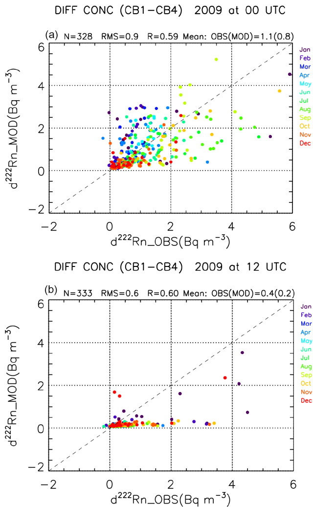
Figure 12. Correlation plots between the simulated (“MOD”) and observed (“OBS”) vertical ^{222}\text{Rn} activity concentration gradients (difference between 20 m (CB1) and 200 m (CB4) at Cabauw at 00:00 UTC (top) and 12:00 UTC (bottom)). Model simulations using InGOS emissions (FI_CT) are shown. Each colour indicates the month at which the data are obtained.
