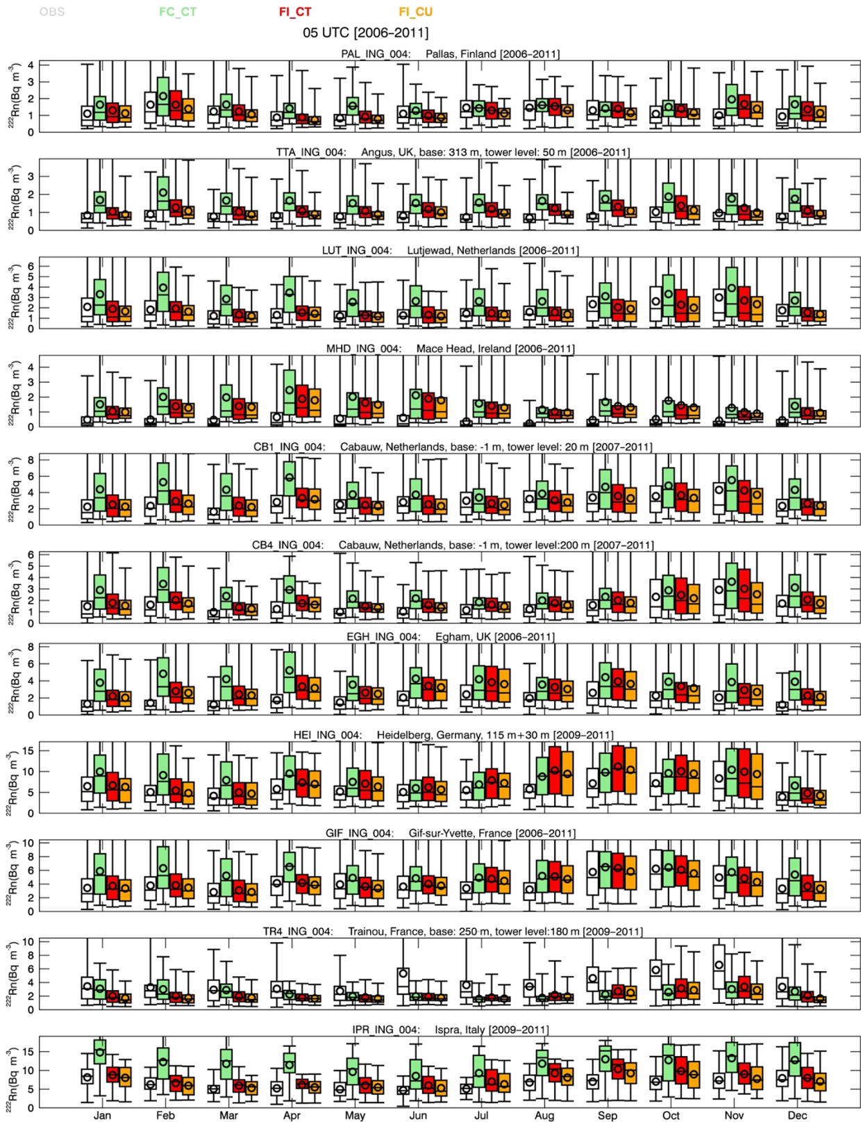
Figure 6. Seasonal variations of daily maximum of observed and simulated radon ( ^{222}\text{Rn} ) activity concentrations at InGOS sites at 05:00 UTC (2006–2011). The whisker plots show the monthly minimum and maximum values (bars), and the 25 and 75 % percentiles (boxes). The median values are given by the horizontal line and the mean values by the open circles in the boxes. The observed radon activity concentrations are shown in blank, and the model simulations are represented by the coloured boxes (the acronyms for the different model simulations are defined in Sect. 3.4). FC uses constant ^{222}\text{Rn} fluxes and FI the InGOS flux map.
