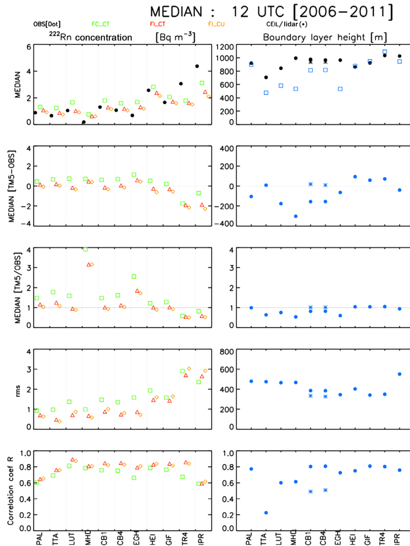
Figure 8. Left: statistics of observed vs. simulated ^{222}\text{Rn} activity concentrations for the different stations (12:00 UTC). Right: statistics of observed (IGRA (●) and ceilometer (CEIL)/lidar (*)) vs. simulated boundary layer heights (TM5_INGOS_IGRA) (12:00 UTC). The acronyms of the stations ( x axis) are given in Table 1. For the median and rms values, the units are given on the top of the two columns.
