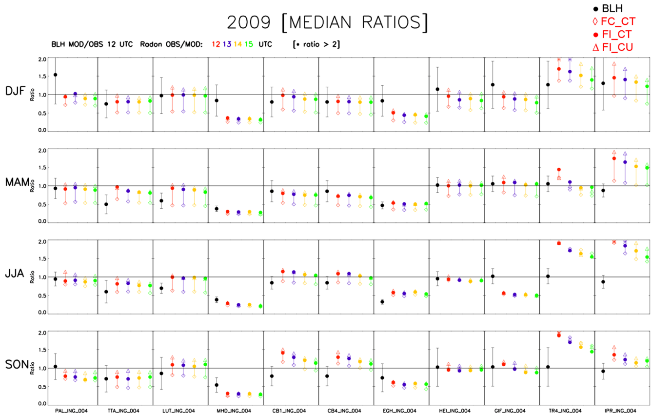
Figure 10. The seasonal variations of the ratios of BLHs (TM5/IGRA; black dots with error bars) at 12:00 UTC and the ratios of ^{222}\text{Rn} activity concentrations (OBS/TM5) at 12:00, 13:00, 14:00, and 15:00 UTC for the four seasons (DJF, MAM, JJA, and SON) of the year 2009 for all InGOS ^{222}\text{Rn} measurement sites. The closest IGRA station to the radon measurement site is considered (see Fig. 1). Three TM5 simulations are shown here: the model simulations using the constant emissions (FC_CT; coloured diamond), InGOS emissions and using the default convection scheme of TM5 (FI_CT; coloured filled circles), and using the new convection scheme (FI_CU; coloured triangles).
