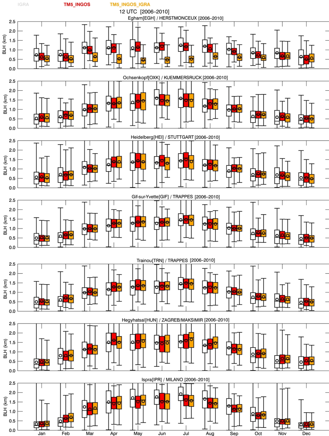
Figure 4. As Fig. 3, but at 12:00 UTC.
