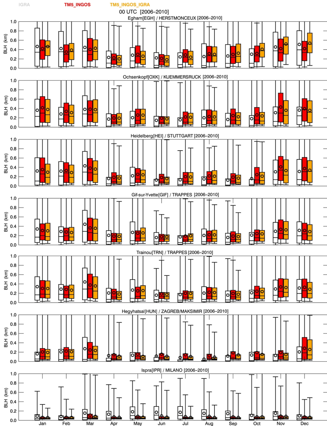
Figure 3. Observed (IGRA; blank) and modelled (TM5_INGOS; red and TM5_INGOS_IGRA; orange) BLHs for InGOS stations at 00:00 UTC (2006–2010). The titles of each panel show the names and acronyms of the InGOS station, and the names of the nearest IGRA station used for comparison. The whisker plots show the monthly minimum and maximum values (bars), and the 25 and 75 % percentiles (boxes). The median values are given by the horizontal line and the mean values by the open circles in the boxes. The different acronyms of the model data are defined in Sect. 3.2 of the text.
