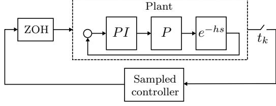
Fig. 2. Sampled-data system setup.
