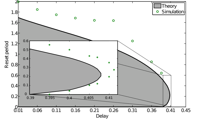
Fig. 3. Example: Maximum and minimum reset period (Prop. 2, N=3 ). Stability proved for a reset period in the shaded area.
