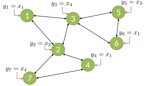
Fig. 3. Network topology in Example 2. The output of the agents are: y_1 = x_1 , y_2 = x_2 , y_3 = x_4 , y_4 = x_1 , y_5 = x_3 , y_6 = x_1 and y_7 = x_4 .
