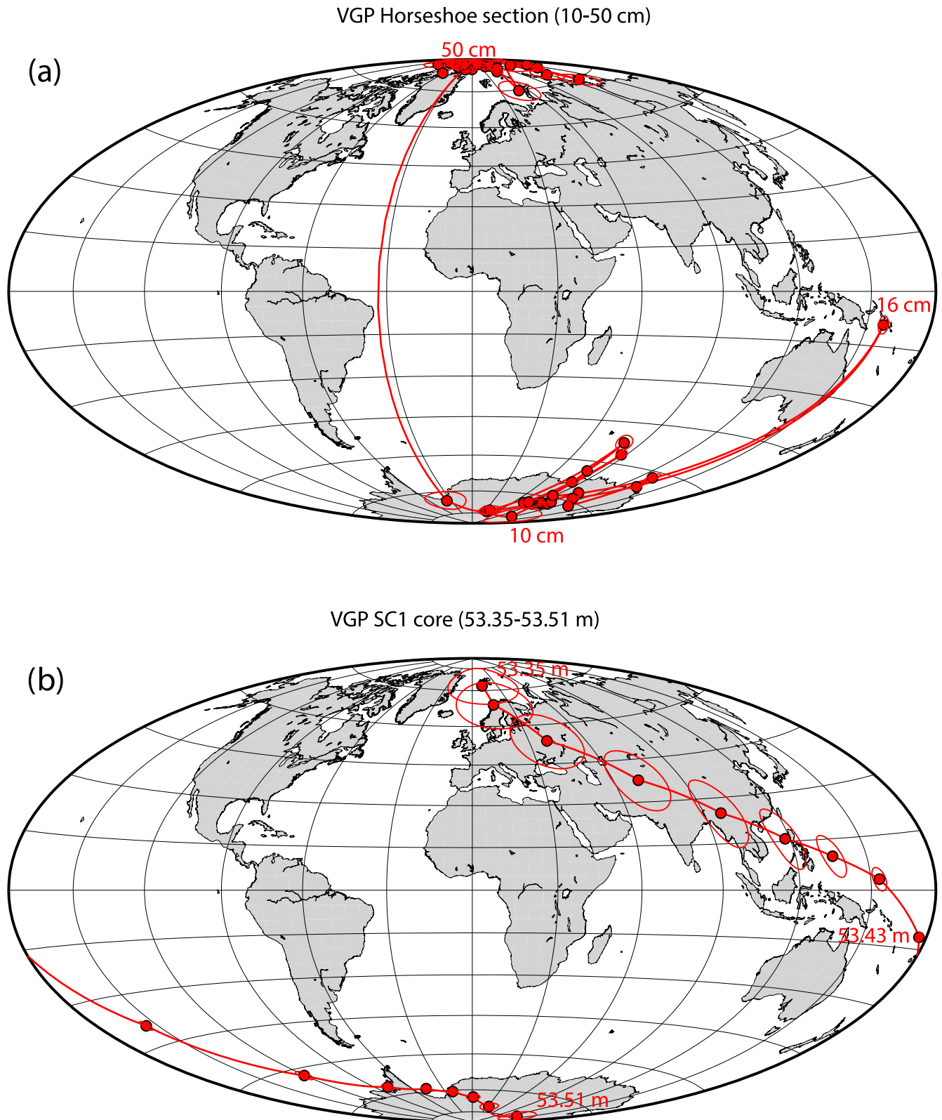
Figure 14. Schematic representation of the VGP path reconstructed from the ChRM directions determined on discrete samples from this study. Ellipses around VGP individual positions represent areas of 95 per cent confidence, that were computed from MAD values about individual ChRM directions. The upper plot (a) refers to VGP reconstructed from ChRM directions determined on discrete samples from this study (the stratigraphic interval in parentheses is referred to this study depth scale; 'd' in Fig. 2). The VGP position near the Solomon Islands (NE of Australia) is related to the large declination swing recorded by the sample centred at a stratigraphic height of 16 cm (Fig. 5). The lower plot (b) refers to VGP reconstructed from ChRM directions determined on u-channel samples collected from core SC1 (authors' unpublished data; declination is arbitrary, the stratigraphic interval in parentheses refers to the SC1 depth scale, indicated as scale 'b' in Fig. 2).
