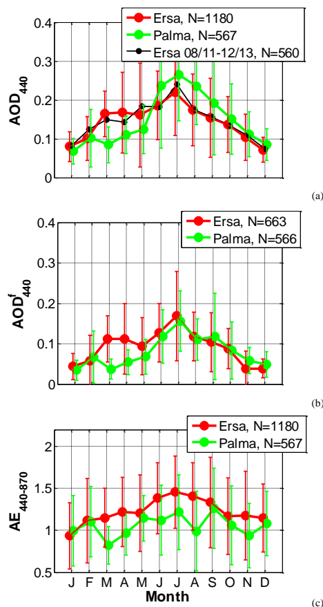
Figure 6. Monthly average variations calculated with daily measurements of (a) aerosol optical depth at 440 nm ( AOD_{440} ), (b) fine-mode aerosol optical depth at 440 nm ( AOD_{440}^f ) and (c) the Ångström exponent calculated between 440 and 870 nm ( AE_{440-870} ) derived from AERONET level 2.0 inversion products available for the period 2011–2015. The error bars represent the standard deviation. On the AOD_{440} plot we have also plotted the monthly values at Ersa calculated over the limited period for which data are also available at Palma, i.e., August 2011–December 2013.
