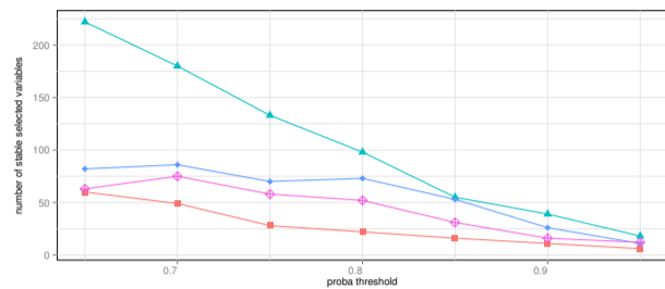
Fig. 1. Number of variables in the set of stable selected variables versus the threshold \pi_{thr} , when forcing the average number of false positives to be smaller than \rho_{error} = 10 . Methods: glmnet (—■—), logit-spls-adapt (—▲—), sgpls (—◆—), spls-log (—◇—). Note: here, all hyper-parameters (including K ) vary across the grid of candidate values \Lambda (c.f. Supp. Mat. section A.6.2).
