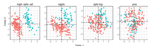
Fig. 2. Observations scores on the first two components for the different methods. The points are shaped according to the value of the response: 0 (●) and 1 (▲). The scores are normalized for comparison.
