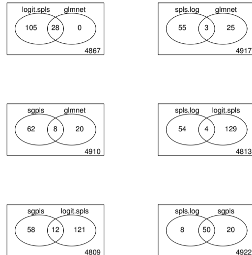
Fig. A.2. Overlap between the genes selected by the different methods thanks to the stability selection procedure, when taking a threshold \pi_{\text{thr}} = 0.75 .
