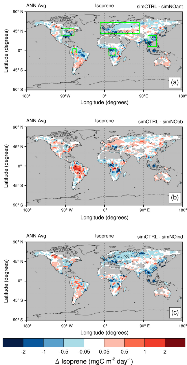
Figure 8. Spatial distribution of annual absolute change in isoprene emission (in \text{mg C m}^{-2} \text{ day}^{-1} ) between the control experiment (SimCTRL) and sensitivity experiments: (a) without all anthropogenic emissions (SimNOant); (b) without biomass burning emissions (SimNObb); and (c) without anthropogenic emissions except biomass burning (SimNOind). All experiments are set in a present-day climatic state. Shaded regions indicate areas where changes in isoprene emission are significant at the 95% confidence level. Green boxes on plot (a) highlight key regions selected for discussion.
