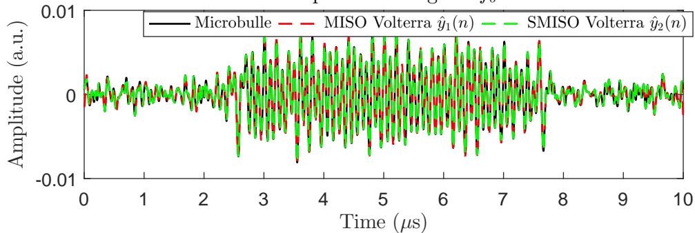
Results from experimental signals f_0 = 10 MHz
