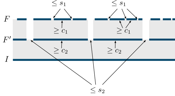
FIGURE 3. A set F of order 2 inside an interval I .
