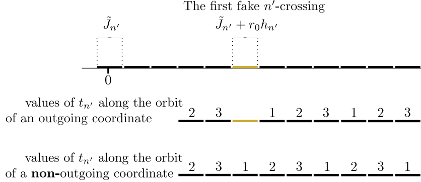
FIGURE 6. The behaviour of t_{n'} along the orbits of outgoing and non-outgoing coordinates
