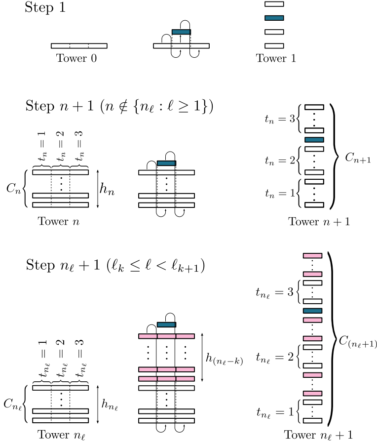
FIGURE 1. Construction of the nearly finite Chacon transformation by cutting and stacking.
