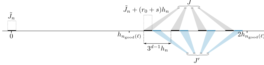
FIGURE 4. The choice of J and J' when n_\ell - \ell < n < n_\ell - k(\ell)
