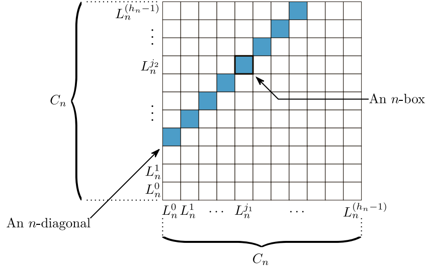
FIGURE 2. An n -diagonal inside C_n^d (here d = 2 )
