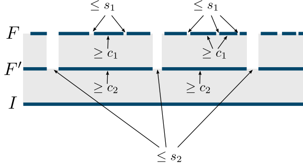
FIGURE 2. A set F of order 2 inside an interval I .
