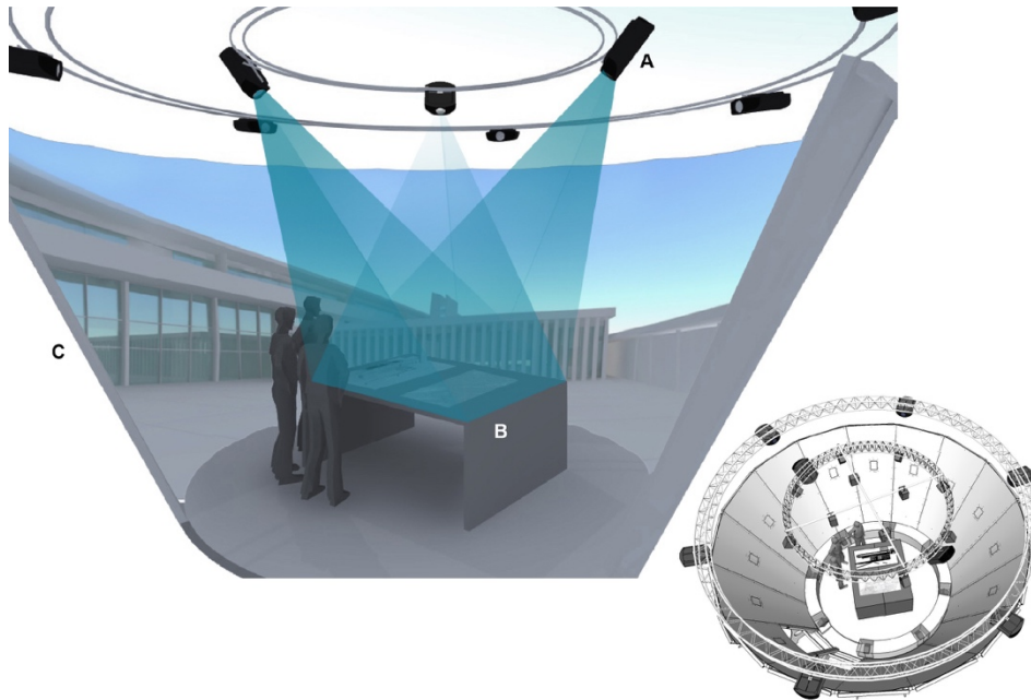
Fig. 01. Possible configuration for CORAULIS (A: 4 beamers for SAR, B: tabletop with augmented plans and mock-up, C: immersive screen) Source: renderings made by the authors.
