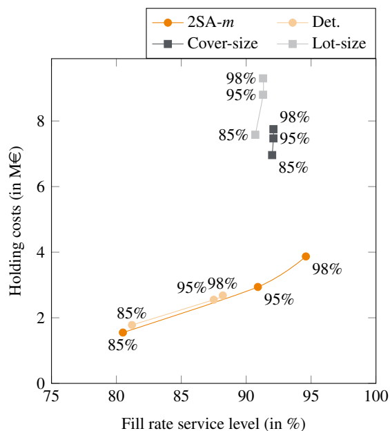
Figure 2: Average results for L2 for various values of desired service level \beta and v = 0.5
