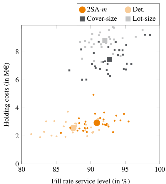
Figure 1: Results for the 30 runs of L2 with v = 0.5 and \beta = 95\%
