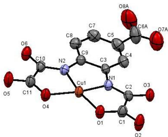
Figure 1. Ellipsoid plot (H and disordered atoms are omitted for clarity) of Cu(L).
