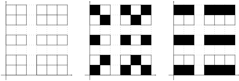
Figure 1. A component from a product of partitions. Left: component \{1, 2, 4, 5, 6\} \times \{1, 2, 4, 6, 7\} . Middle: alternating assignment rule of 1 (black) and -1 (white) values. Right: mixture of identical assignment rule in horizontal direction and alternating assignment rule in vertical direction.
