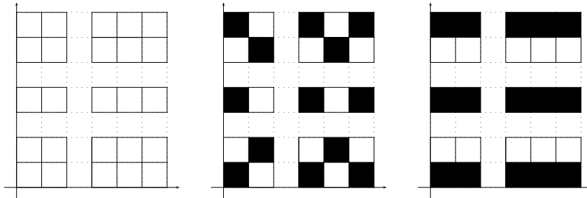
FIGURE 1. A component from a Cartesian product of partitions. Left: component \{1, 2, 4, 5, 6\} \times \{1, 2, 4, 6, 7\} . Middle: alternating assignment rule of 1 (black) and -1 (white) values. Right: mixture of identical assignment rule in horizontal direction and alternating assignment rule in vertical direction.
