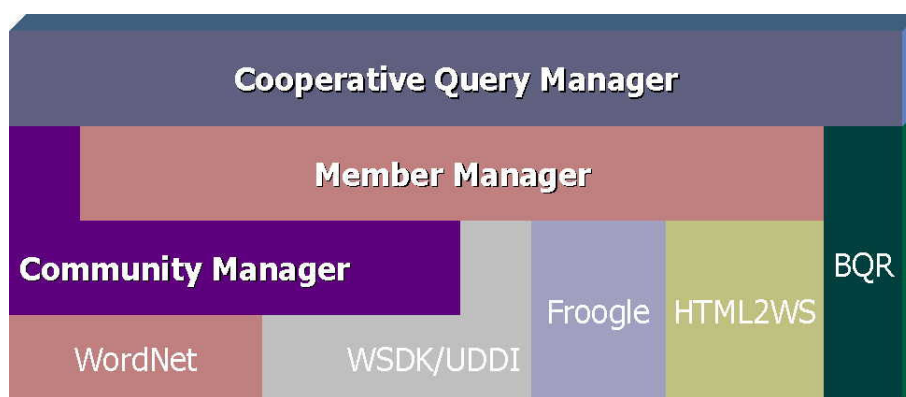
Fig. 4. WS-CatalogNet Architecture
