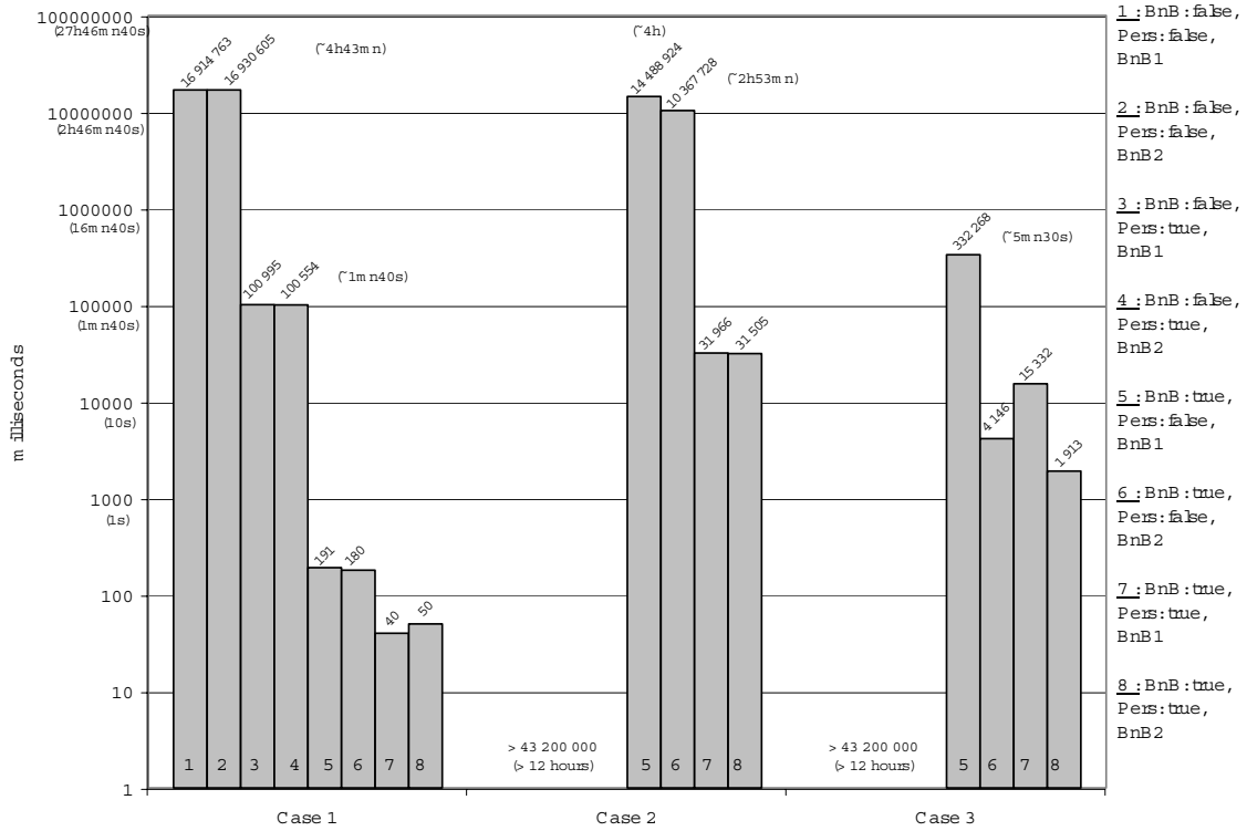
Fig. 5. Execution time
