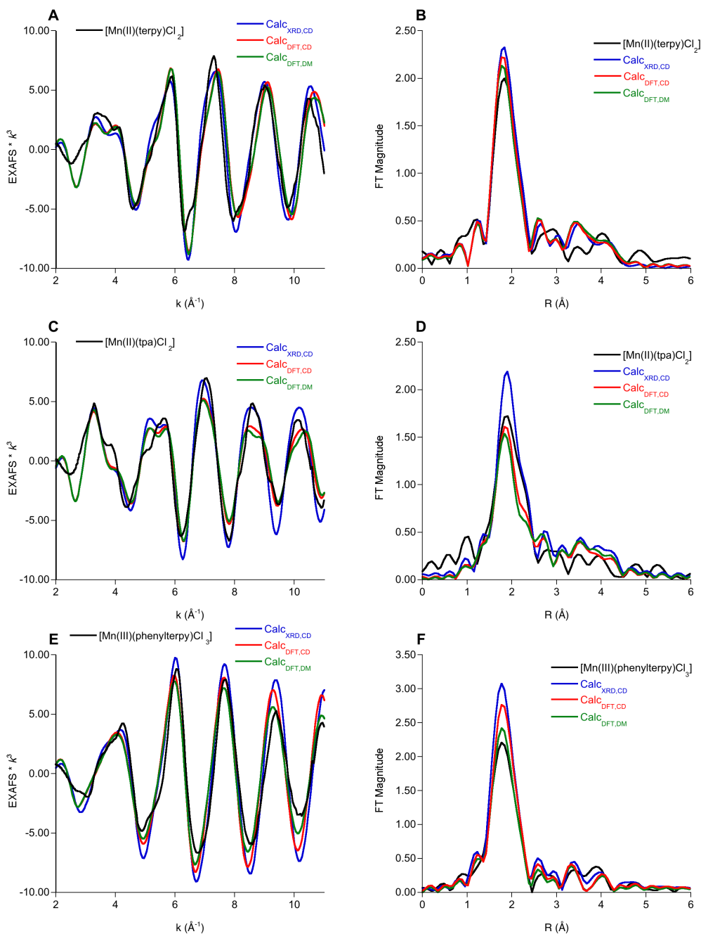
Figure 2. Experimental (black) and theoretical \chi(k) spectra calculated using FEFF 9.1 and the corresponding non phase shift corrected FTs of [\text{Mn(II)(terpy)Cl}_2] (A and B), [\text{Mn(II)(tpa)Cl}_2] (C and D), and [\text{Mn(III)(phenylterpy)Cl}_3] (E and F). The calculations for the spectra using the \text{Calc}_{\text{DFT,CD}} method included Debye temperatures determined using the sum of the first shell Mn-L stretching frequencies.
