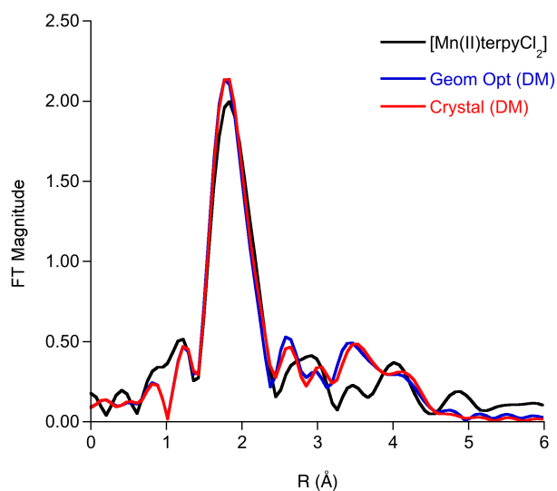
Figure S2. Non phase shift corrected FTs of the experimental (black) and theoretical EXAFS using the DM method at the geometry optimized (blue) and at the crystal (red) structure coordinates of [Mn(II)(terpy)Cl 2 ].
