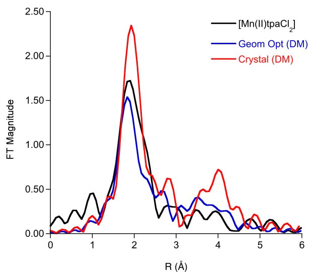
Figure S3. Non phase shift corrected FTs of the experimental (black) and theoretical EXAFS using the DM method at the geometry optimized (blue) and at the crystal (red) structure coordinates of [Mn(II)(tpa)Cl 2 ].
