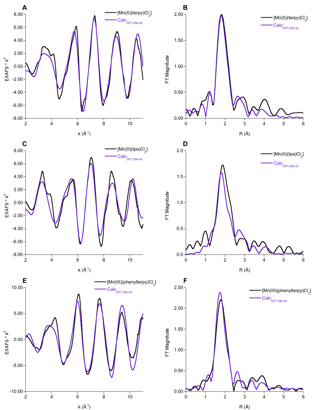
Figure S8. Experimental (black) and Calc DFT,DM-ref fits (purple) to the \chi(k) spectra and the corresponding non phase shift corrected FTs of [Mn(II)(terpy)Cl 2 ] (A and B), [Mn(II)(tpa)Cl 2 ] (C and D), and [Mn(III)(phenylterpy)Cl 3 ] (E and F).
