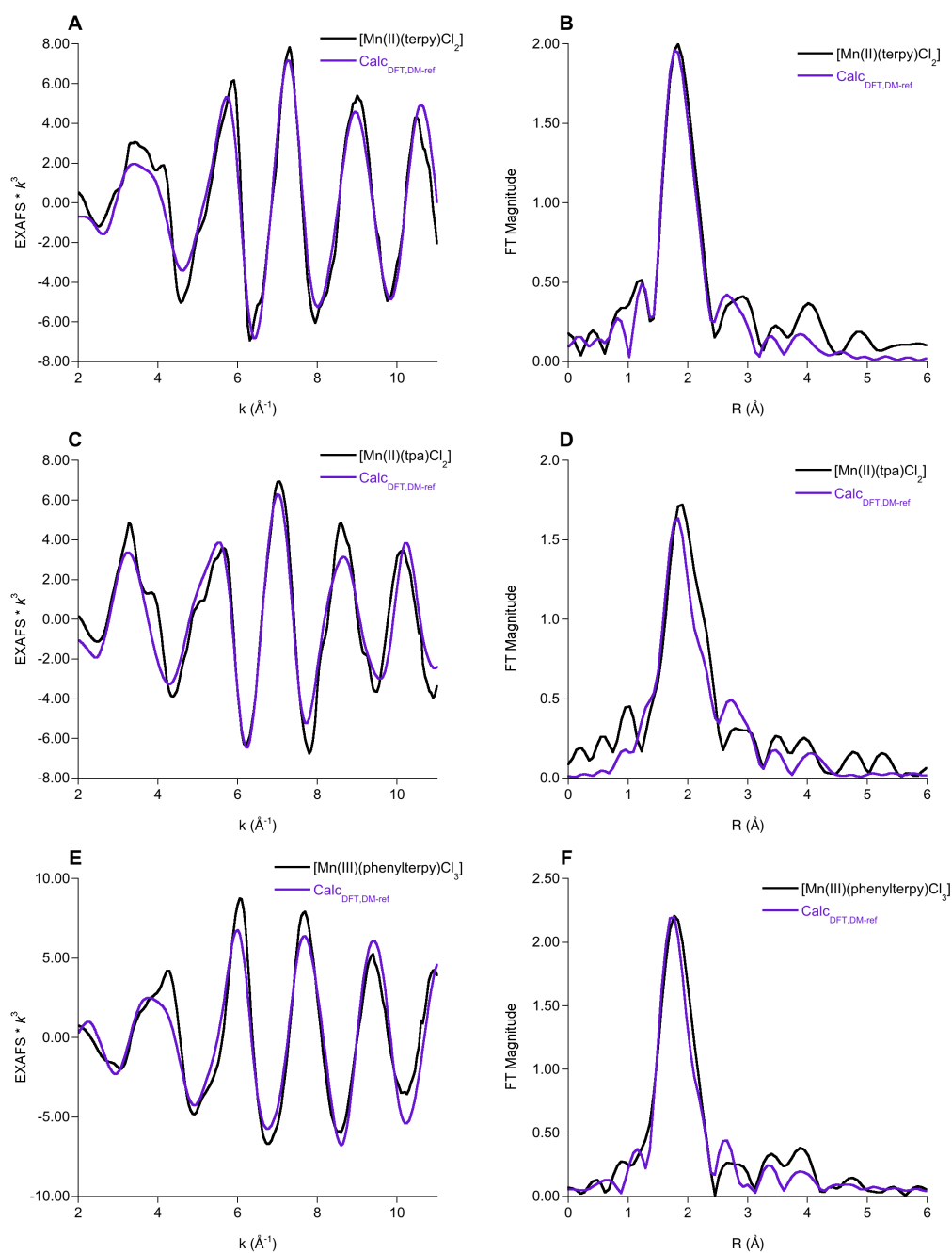
Figure S14. Experimental (black) and Calc DFT,DM-ref fits (purple) to the \chi(k) spectra allowing S_0^2 to refine and the corresponding non phase shift corrected FTs of [Mn(II)(terpy)Cl 2 ] (A and B), [Mn(II)(tpa)Cl 2 ] (C and D), and [Mn(III)(phenylterpy)Cl 3 ] (E and F).
