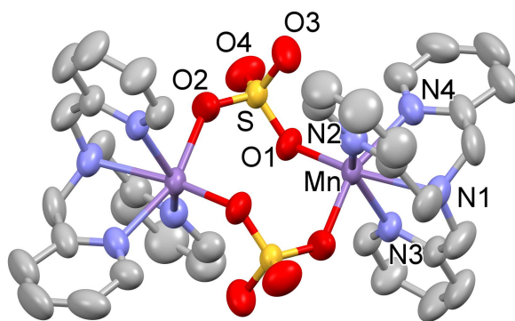
Figure S1. ORTEP diagram showing the molecular structure of [\text{Mn}_2(\text{II})(\mu\text{-SO}_4)_2(\text{tpa})_2] . Hydrogen atoms and solvent molecules have been omitted for clarity.
