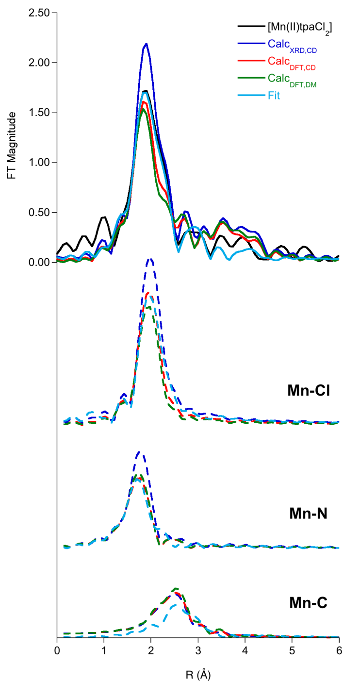
Figure 3. Calculated spectra and contributions of significant single scattering paths to the total spectra for [Mn(II)(tpa)Cl 2 ]. The deconvolutions for each method are the sums of the individual scattering paths of each type. The calculations for the spectra using the Calc DFT,CD method included Debye temperatures determined using the sum of the first shell Mn-L stretching frequencies. Spectra have been offset on the y-axis, but share a common y-scale.
