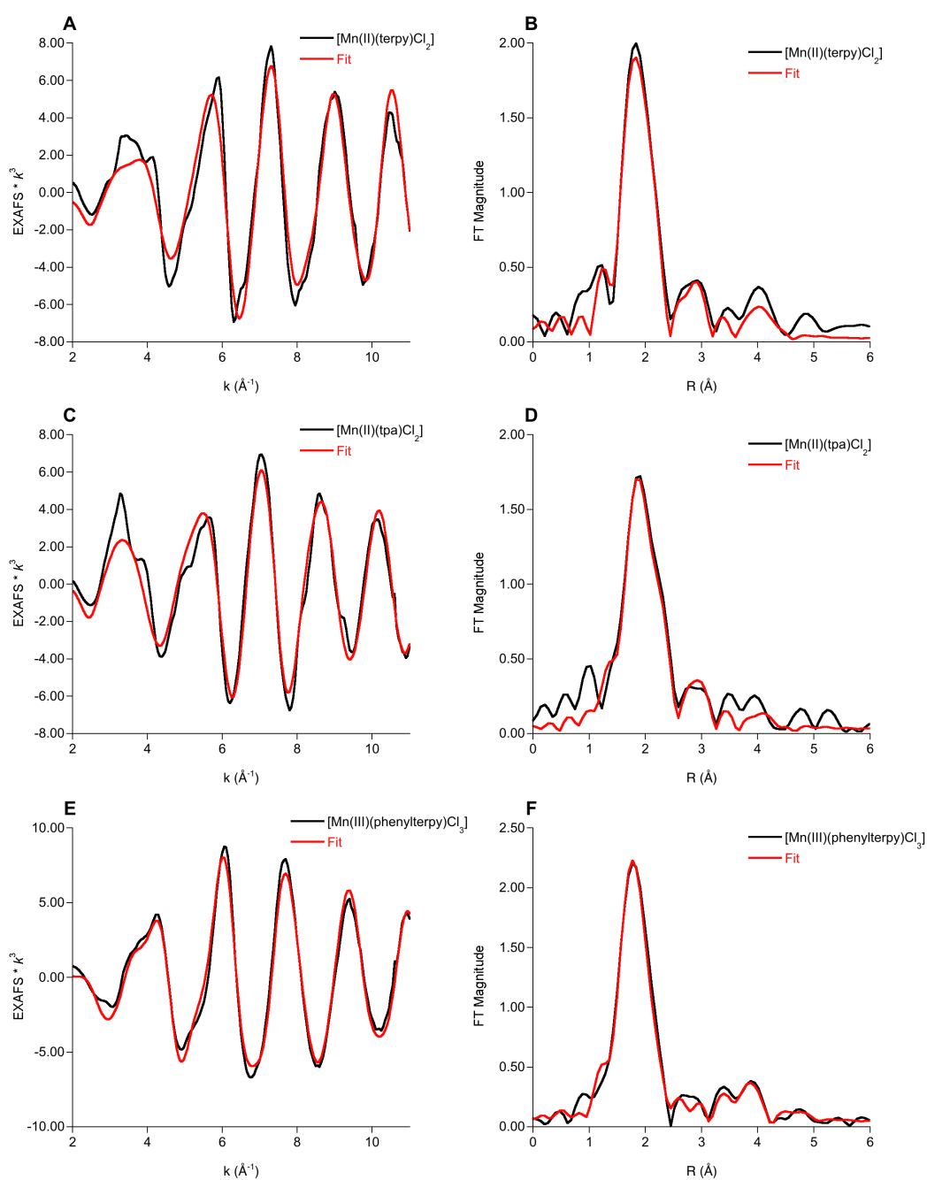
Figure S10. Experimental (black) and fits (red) to the \chi(k) spectra allowing S_0^2 to refine and the corresponding non phase shift corrected FTs of [Mn(II)(terpy)Cl 2 ] (A and B), [Mn(II)(tpa)Cl 2 ] (C and D), and [Mn(III)(phenylterpy)Cl 3 ] (E and F).
