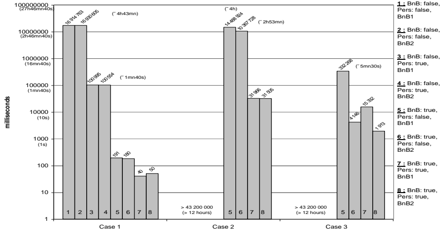
Figure 3: Execution time
