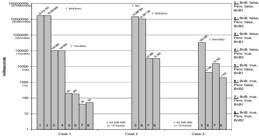
Figure 3: Execution time
