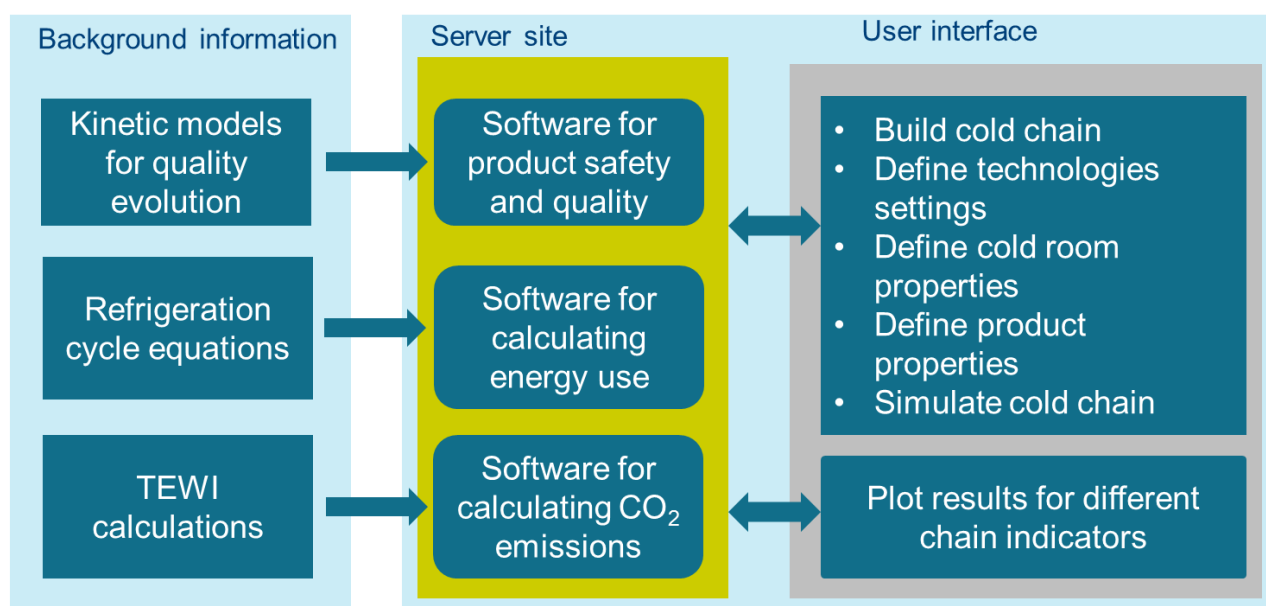
Figure 1. Main components of QEEAT 4.0
