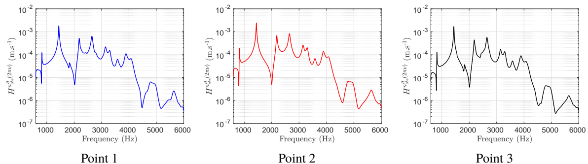
Figure 14 – Elevation \nu \mapsto H_{obs}^H(2\pi\nu) of the observation points n_{obs}^H = (1, 2, 3) on the free surface (left, middle, right).
