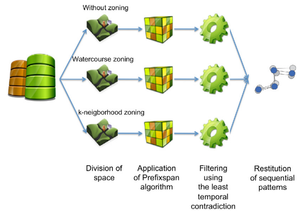
Figure 2: Process of knowledge discovery applied to hydrologic network.
