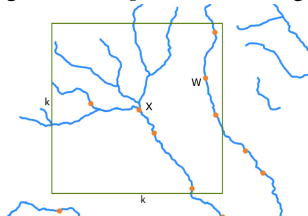
Figure 4: k -neighborhood zoning.
